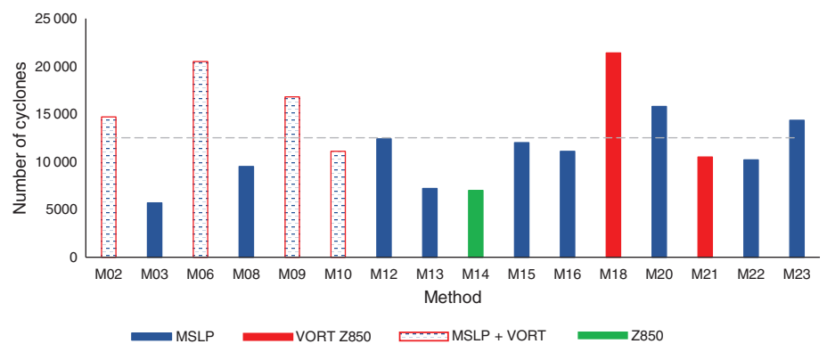
Figure 2. The number of Northern Hemisphere ( 30^\circ – 90^\circ N), winter (December, January and February) cyclones between 1989 and 2009, using 16 different tracking methods. Adapted from Table 2 in Neu et al. (2013), with the addition of M23, representing the results from Massey's (2016) tracking algorithm. Grey dashed line represents the mean, with shading representing the primary variable used for identification – blue represents MSLP, red represents relative vorticity at 850hPa (VORT Z850), hatched represents MSLP and/or Laplacian of MSLP or vorticity (VORT), and green represents geopotential height at 850hPa (Z850). (Source: Neu et al. , 2013.)
