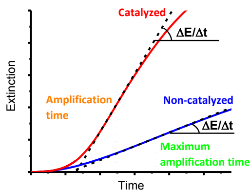
Figure 2. Schematic representation of time-dependent extinction measurements of precipitation polymerizations to illustrate assay results for a catalyzed (red curve) and a non-catalyzed reaction (blue curve). The rate of turbidity formation ( \Delta E/\Delta t ) is calculated by linear regression (black dashed lines) over the quasi-linear increase of extinction. The amplification time (orange and green dotted lines) correspond to the minimal time needed to reach maximum \Delta E/\Delta t . The maximum amplification time (green dotted line) is the time needed for the non-catalyzed reaction to reach maximum \Delta E/\Delta t .
