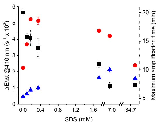
Figure 6. Influence of concentration of sodium dodecyl sulfate on the rate of turbidity formation for precipitation polymerizations catalyzed by 100 ng mL -1 sHz (red dot) and non-catalyzed reactions (blue triangle) (average of n = 3 and SD). The amplification time of the non-catalyzed reaction (grey square, average of n = 3 and SD) is displayed on the second y axis (grey square). Reaction conditions were 800 mM NIPAAm, 36 mM HEBIB, 80 mM Asc, 45 °C and pH 7.
