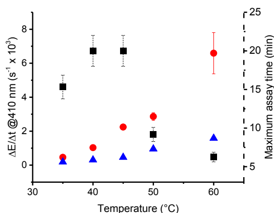
Figure 8. Influence of temperature on the rate of turbidity formation for precipitation polymerizations catalyzed by 100 \text{ ng mL}^{-1} \text{ sHz} (red dot) and non-catalyzed reactions (blue triangle) (average of n = 3 and SD). The amplification time of the non-catalyzed reaction is displayed on the second y axis (grey square, average of n = 3 and SD). Reaction conditions: 800 mM NIPAAm, 36 mM HEBIB, 80 mM Asc, 170 \mu\text{M} SDS and pH 7.
