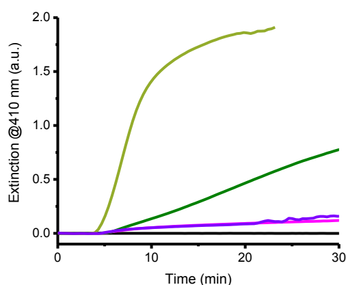
Figure 4. Contribution of individual reagents on the precipitation polymerization. Normal catalyzed reaction condition (pale green, 800 mM NIPAAm, 36 mM HEBIB, 80 mM Asc, 170 \mu M SDS, 100 ng mL -1 sHz, 45 ^{\circ} C, pH 7), non-catalyzed reaction (dark green), catalyzed reaction without HEBIB (purple), non-catalyzed reaction without HEBIB (pink), and non-catalyzed reaction without sodium ascorbate (black).
