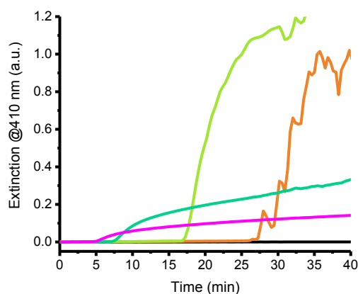
Figure 5. Contribution of ascorbate and oxygen to the non-catalyzed precipitation polymerization. Sodium ascorbate concentrations were investigated at 0 mM (black), 4 mM (orange), 8 mM (pale green), 40 mM (green) and 80 mM (pink). Reaction conditions: 800 mM NIPAAm, 0 mM HEBIB, 170 \mu M SDS, no sHz, 45 ^{\circ} C, pH 7. Please note: This noisy signal arises when PNIPAAm particles sediment, i.e. when larger polymer particles form.
