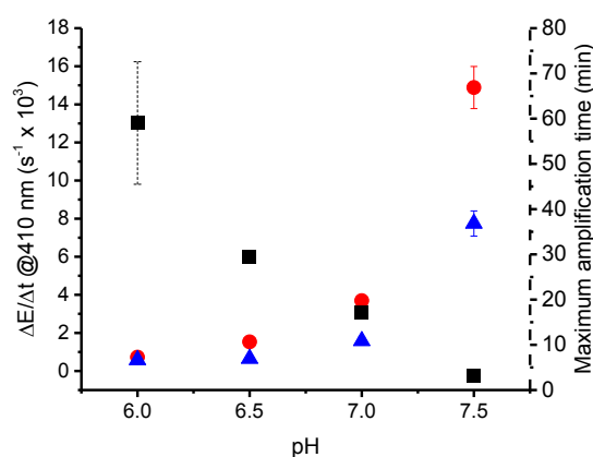
Figure 9. Effect of pH on the rate of turbidity formation for precipitation polymerizations catalyzed by 100\text{ ng mL}^{-1} sHz (red dot) and non-catalyzed reactions (blue triangle) (average of n = 3 and SD). The amplification time of the non-catalyzed reaction is displayed on the second y axis (grey square, average of n = 3 and SD). Reaction conditions: 800\text{ mM NIPAAm} , 36\text{ mM HEBIB} , 80\text{ mM Asc} , 170\text{ }\mu\text{M SDS} and 45^\circ\text{C} .
