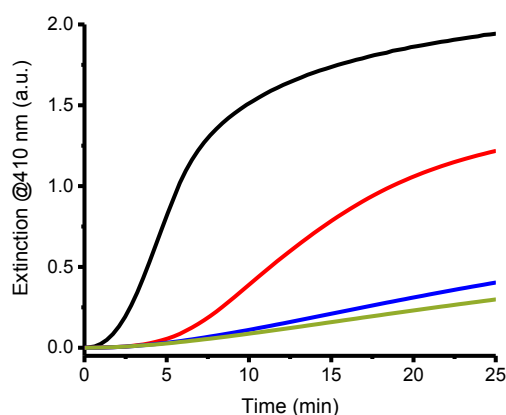
Figure 3. Influence of the presence of oxygen on the hemozoin-catalyzed precipitation polymerization. Reaction catalyzed by 100 \text{ ng mL}^{-1} sHz purged with argon (black line) and non-degassed (red curve) are
