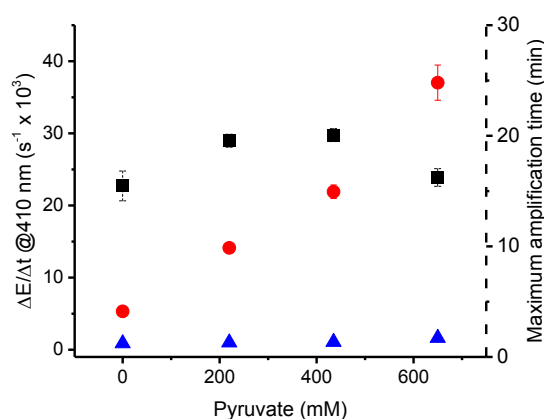
Figure 7. Impact of the pyruvate concentration on the rate of turbidity formation for precipitation polymerizations catalyzed by 100 \text{ ng mL}^{-1} sHz (red dot) and non-catalyzed reactions (blue triangle) (average of n = 3 and SD). The amplification time of the non-catalyzed reaction (grey square, average of n = 3 and SD) is displayed on the second y axis. Reaction conditions: 800 mM NIPAAm, 36 mM HEBIB, 80 mM Asc, 170 \mu\text{M} SDS, 45 ^\circ\text{C} , pH 7.
