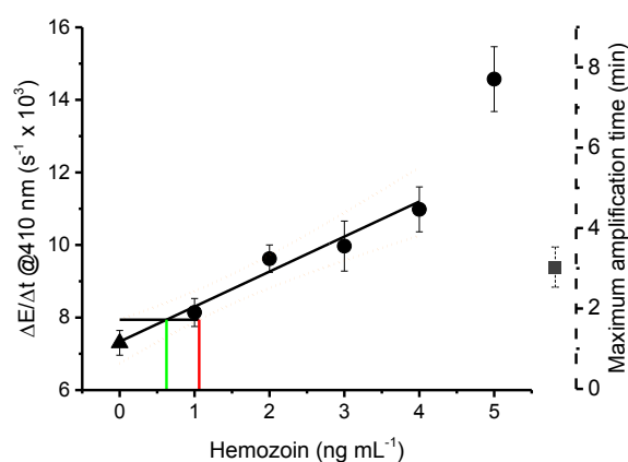
Figure 10. Dose-response curve of the optimized hemozoin-catalyzed precipitation polymerization assay at low concentrations of synthetic hemozoin (average of n = 5 and SD, linear data fit (black line), 95 % confidence interval (orange dotted line), decision limit (green vertical line) and limit of detection (red vertical line)). Maximum amplification time, i.e. the time of the non-catalyzed reaction is displayed on the second y axis (grey square, average of n = 5 and SD). Reaction conditions were 800 mM NIPAAm, 36 mM HEBIB, 80 mM Asc, 650 mM Pyr, 170 \mu\text{M} SDS, 45 °C and pH 7.5.
