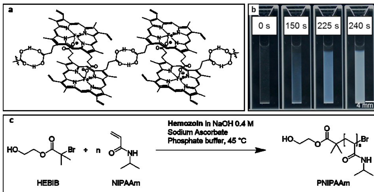
Figure 1 Hemozoin-catalyzed precipitation polymerization of NIPAAm. a Scheme of crystal structure of hemozoin. b Turbidity formation during an assay catalyzed by 100 ng mL -1 of synthetic hemozoin (800 mM NIPAAm, 36 mM HEBIB, 80 mM Asc, 650 mM Pyr, 170 μM SDS, 45 °C and pH 7.5) over time. c Reaction scheme of the polymerization.
