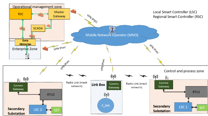
Fig. 1 LV Engine SCS high Level communication architecture
