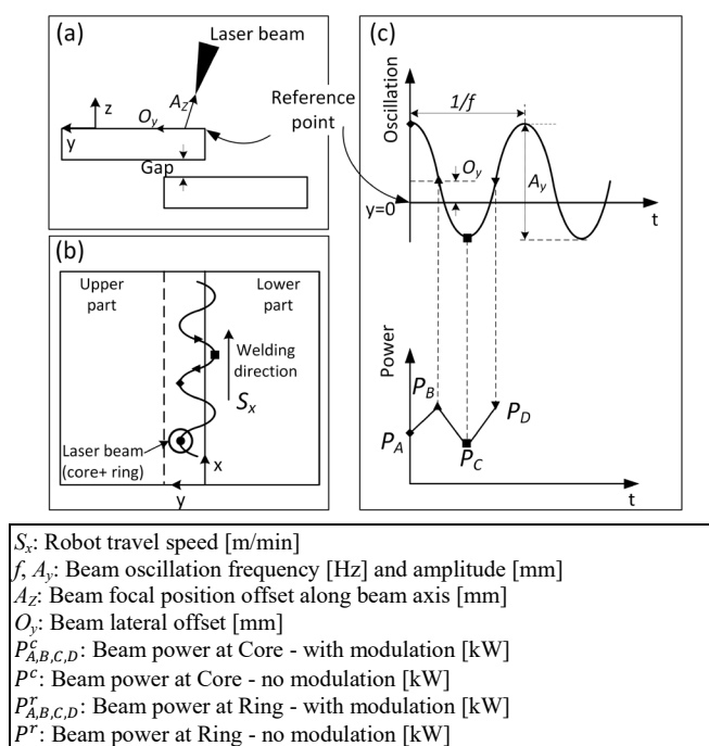
Fig. 3. Illustration of key welding parameters; (a) cross view; (b) top view and; (c) beam oscillation and power modulation [9].
