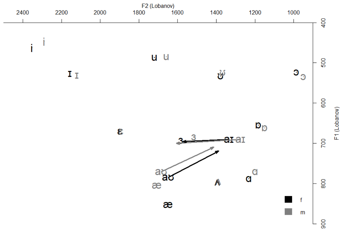
Figure 5. F1-F2 formant frequency plots showing trajectories of participants' productions of the PRICE and MOUTH vowels, measured at 20% and 80% of the vowel duration and averaged across gender (f= female, m = male). There were no significant gender differences for either of these vowels.
