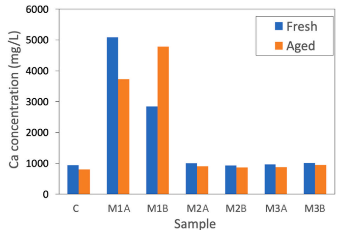
Fig. 7. Calcium concentration measured by ICP-OES in solutions in equilibrium with the putties.
