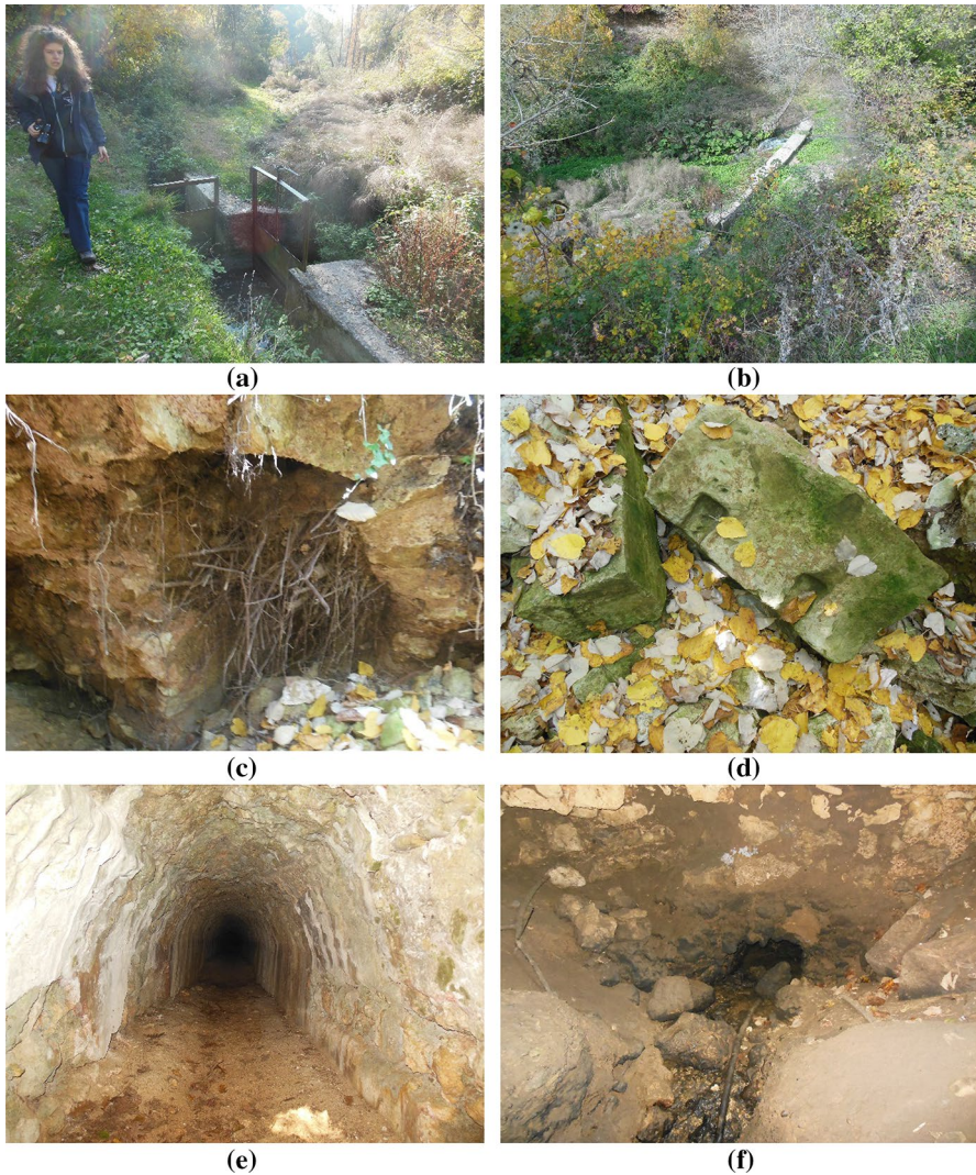
Fig. 6 Modern weir and sluice arrangement near intake at Pazarlı (a, b), the inlet to the aqueduct channel being hidden in the undergrowth behind Dr Ruggeri in (a); and springs at Pinarca showing aqueduct channel (c) and fallen masonry that may have been a weir of Roman construction (d) at the first spring; well-preserved channel at the second spring (e); and channel (with a modern water pipe fed through it) at base of weir at the third spring (f)
