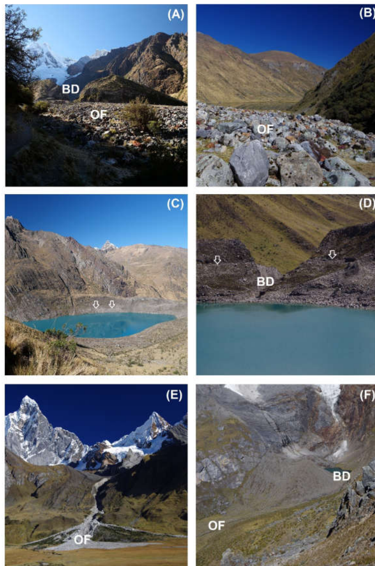
Figure 3. Examples of diagnostic features of past glacial lake outburst floods (GLOFs) in the Cordillera Huayhuash. (A) Upstream view on breached moraine dam (BD) of Lake Solteracocha (in centre background) with outwash fan located directly downstream from the dam (OF); (B) downstream view over this outwash fan (OF), the largest boulders are > 2 m in diameter; (C) visible evidence of Solteracocha pre-GLOF lake water level (arrows; GLOF in 1932); (D) downstream view
