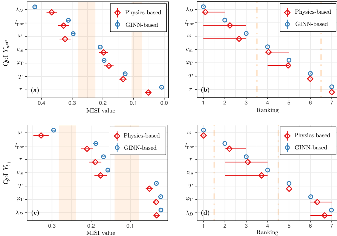
Figure 2: Plug-in Monte Carlo estimators of the first-order MISIs in (4) indicate the most impactful CVs X for tuning the QoIs Y_{\kappa^{\text{eff}}} (top row) and Y_{t_+} (bottom row). For Algorithm 1 (left column), the width of the confidence intervals (23) is chosen to achieve a non-overlap significance level \bar{\gamma} = 0.01 pairwise on average. The highlighted gaps in (a) and (c) indicate clusters of CVs with similar relative importance. For Algorithm 2 (right column), the GINN-based estimators for CV ranking with percentile confidence intervals (27) are consistent with the rankings in (a) and (c). These ranks are resolved, which is not feasible through bootstrapping the 3 \times 10^3 samples from the physics-based model. In both algorithms, the GINN surrogate enables querying sufficiently large amounts of data to distinguish closely-ranked CVs with a high degree of confidence. In (b) and (d) the dashed lines correspond to the gaps identified in (a) and (c), respectively.
