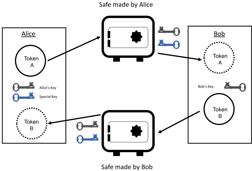
Fig. 2 An example of atomic swap
