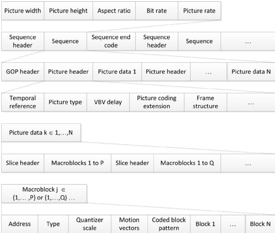
Figure 3-7. Structure of MPEG-2 video bitstream syntax
