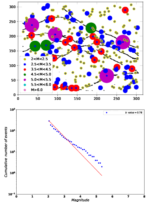
Figure 16. (a) Example of the spatial distribution of simulated events for a particular FBM realization with P = 0 , \pi_{\text{frac}} = 0.95 , and N = 300 . Circular areas depict the equivalent magnitude–area relation computed from Eq. (6). Star markers indicate the epicenter of each simulated earthquake. (b) Gutenberg–Richter fit of simulated events ( P = 0 , \pi_{\text{frac}} = 0.95 , \pi_{\text{bkg}} = 0.65 , and N = 300 ).
