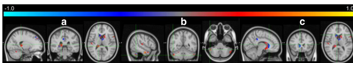
Fig. 10 Differences between statistical maps of the HE model using GLM and GAM at different brain ROIs: right hippocampus (A), right caudate (B) and right cerebellar crus (C). A positive (negative) value indicates that GAM (GLM) is statistically better using the f-test metric
