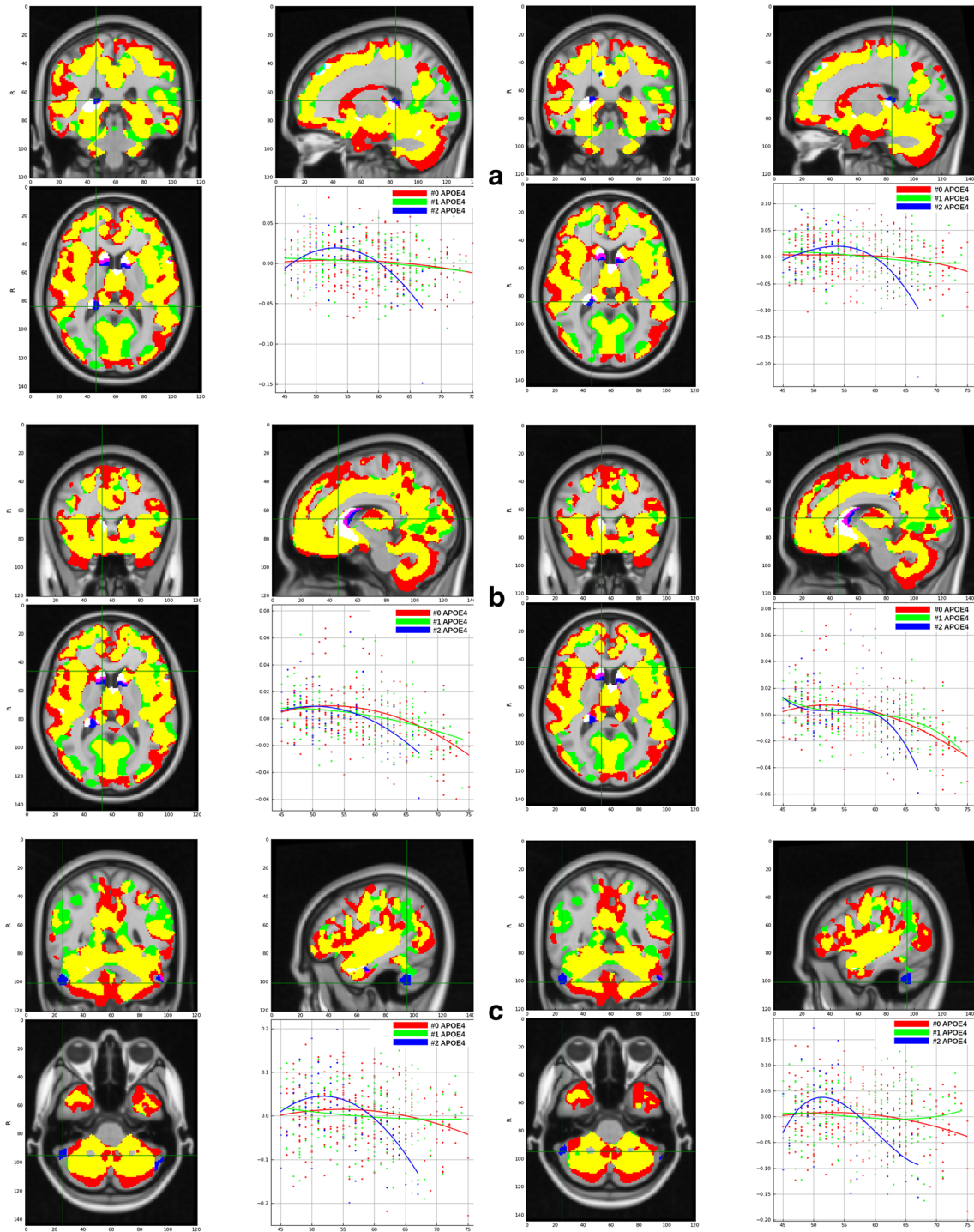
Fig. 9 Interaction between age and the APOE- \epsilon 4 genotype using second order polynomial expansion of GLM (left) and B-splines GAM (right). Three different regions are shown at each row: (A) right hippocampus, (B) right caudate and (C) right cerebellar crus. Statistical analysis using F-test and uncorrected p < 0.001 threshold with cluster size of 100 voxels.
