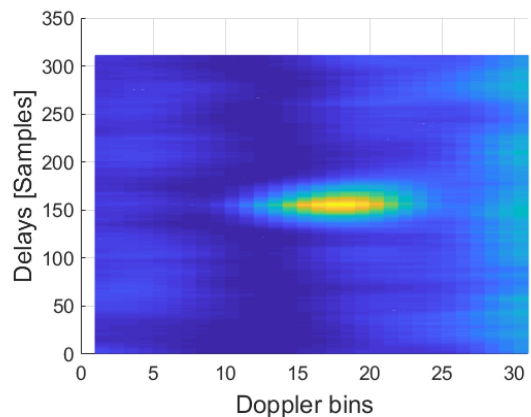
Fig. 8. Example DDM from of 1 ms coherent of GPS L1 C/A build from 31 Doppler slices (WF). Reflection over the sea.
