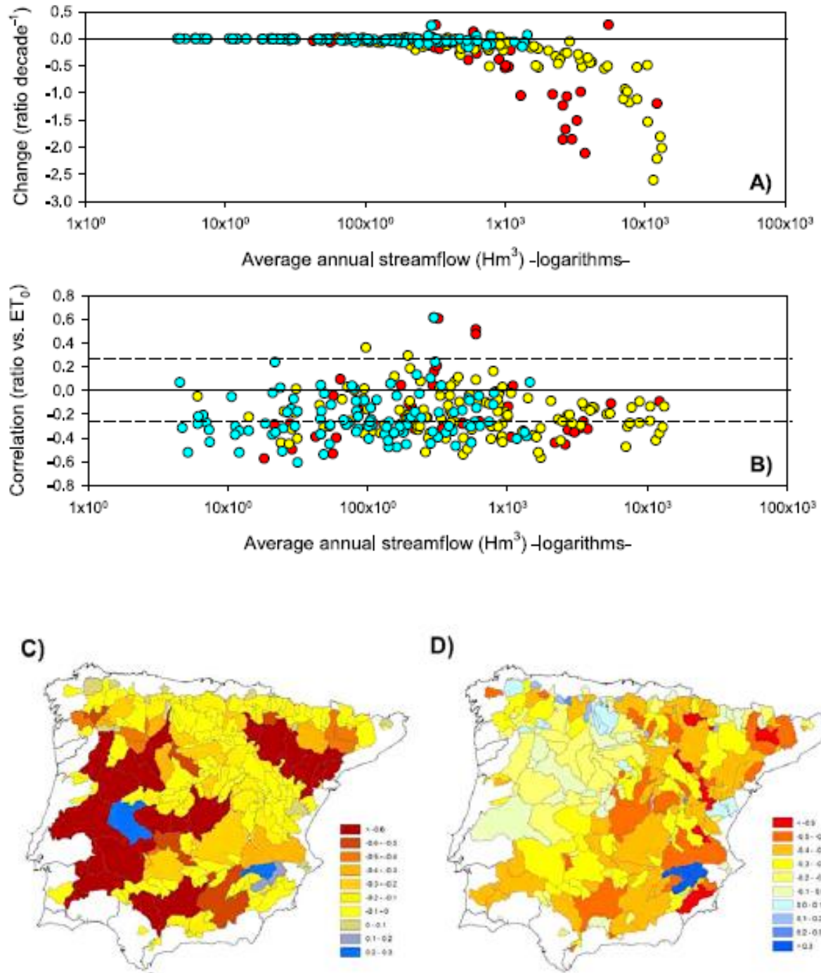
Figure 39: (a) Magnitude of change in the streamflow/precipitation ratio for Iberian peninsula, 1961-2009 (Vicente-Serrano et al., 2014). (b) shows the Pearson's r correlation between the annual streamflow/ precipitation ratio and evapotranspiration ( ET_0 ), dotted lines indicating the limits of significance. (c) and (d) show the spatial distribution of the magnitude and the correlation respectively.
