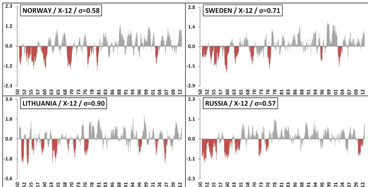
Figure 35a: Northern Europe country drought series for the period 1950–2012 according to the indicator X-12 for some selected countries (drought events are marked in red). X-12 represents an index based on the average of values for SPI, SPEI and RDI accumulated over 12-months.
