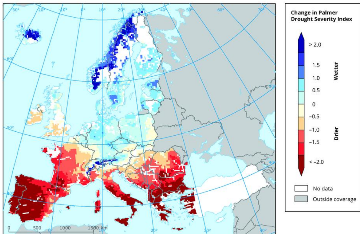
Figure 45: Projected changes in summer soil moisture between the periods 1961 to 1990 (baseline) and 2021 to 2050 (scenario) 37
