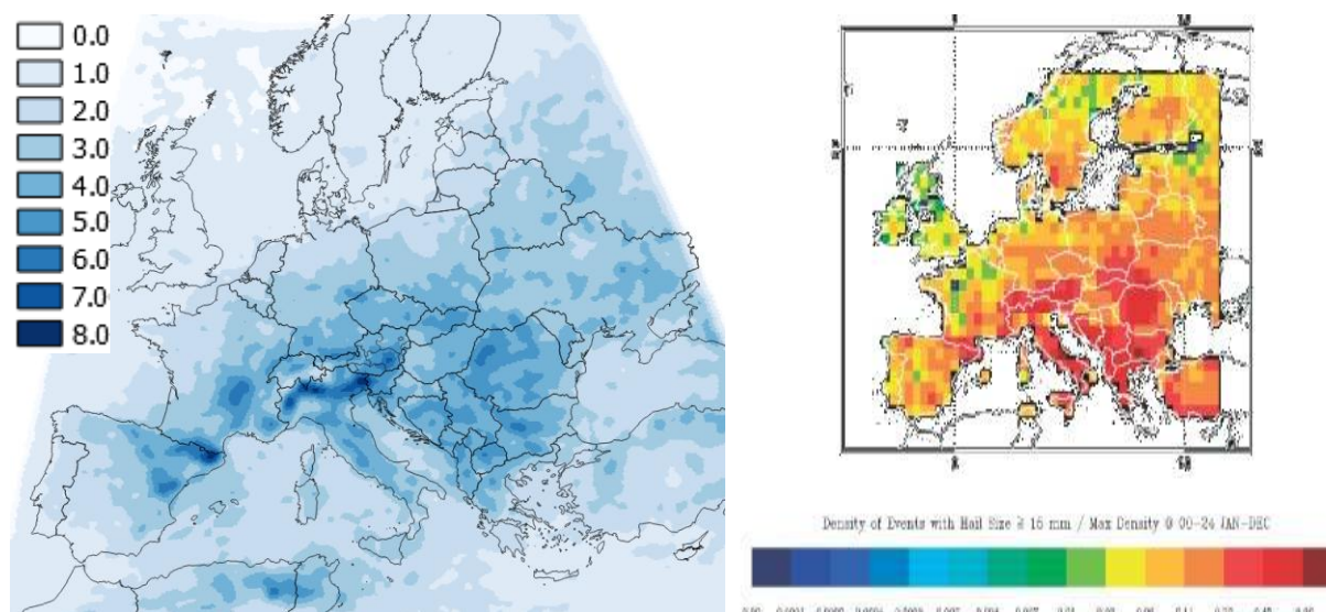
Figure 56: Comparison between (a) OT-based climatology (occurrences per year and 100 km 2 ) and (b) Hail day density (Hand and Cappelutti, 2011).
