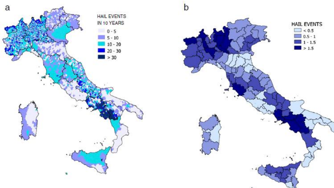
Figure 30: Distribution of hail events: a) decadal distribution at municipality scale; b) yearly distribution at provincial scale (Baldi et al., 2014).
