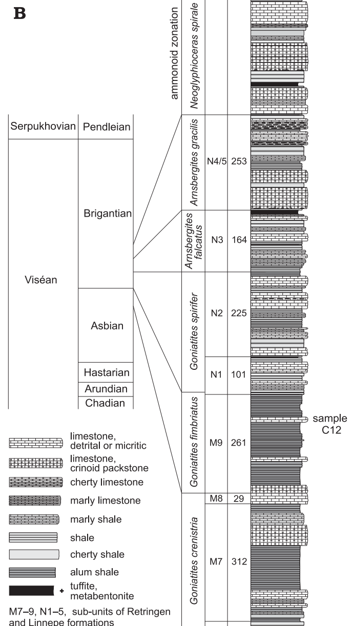
Fig. 3. A. Position of Westenfeld Quarry against the outline of Mississippian outcrops in the northern Rhenish Mountains. B. Fragment of the stratigraphic column of the Westenfeld Quarry showing position of sample C12, studied in this paper.
