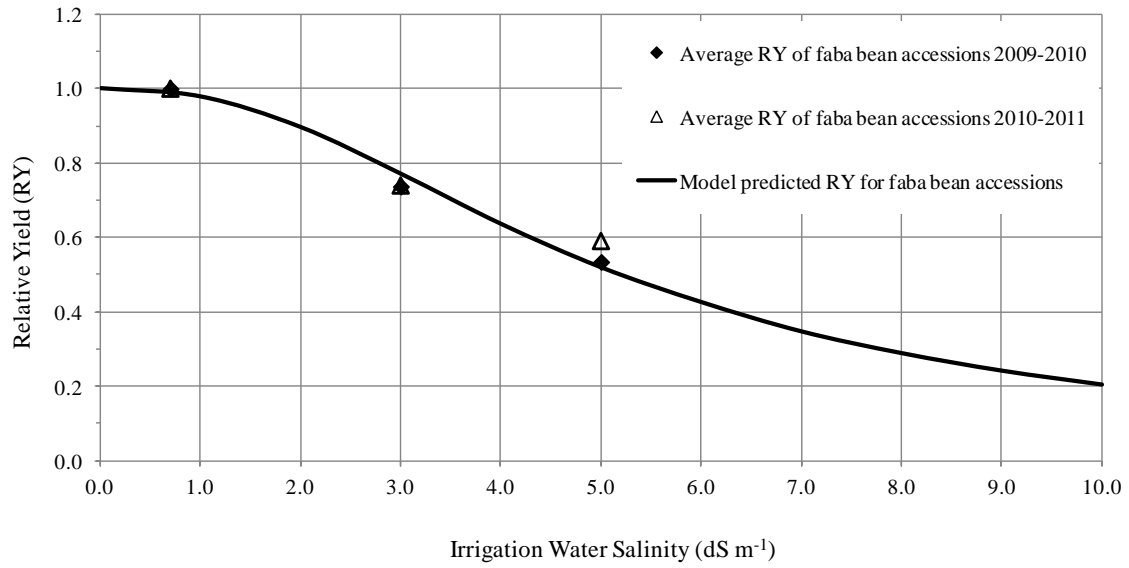
Figure 3. As predicted and validated by SALTMED model, decrease in relative grain yield of Faba bean as affected by the incremental increase in irrigation water salinity up to 10 dS m -1
