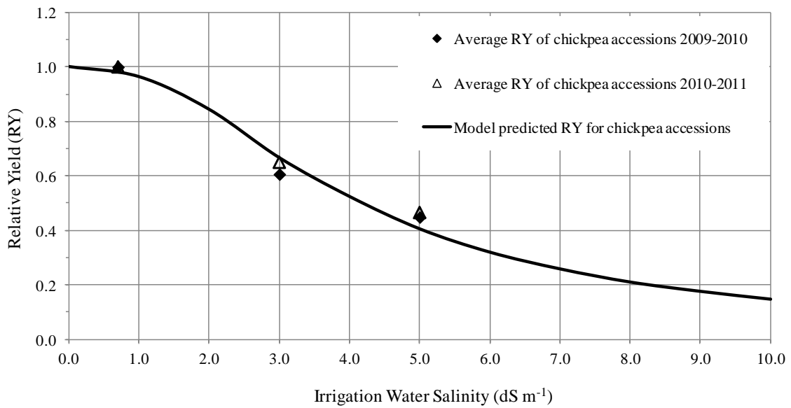
Figure 2. As predicted and validated by SALTMED model, decrease in relative grain yield of Chickpea as affected by the incremental increase in irrigation water salinity up to 10 dS m -1
