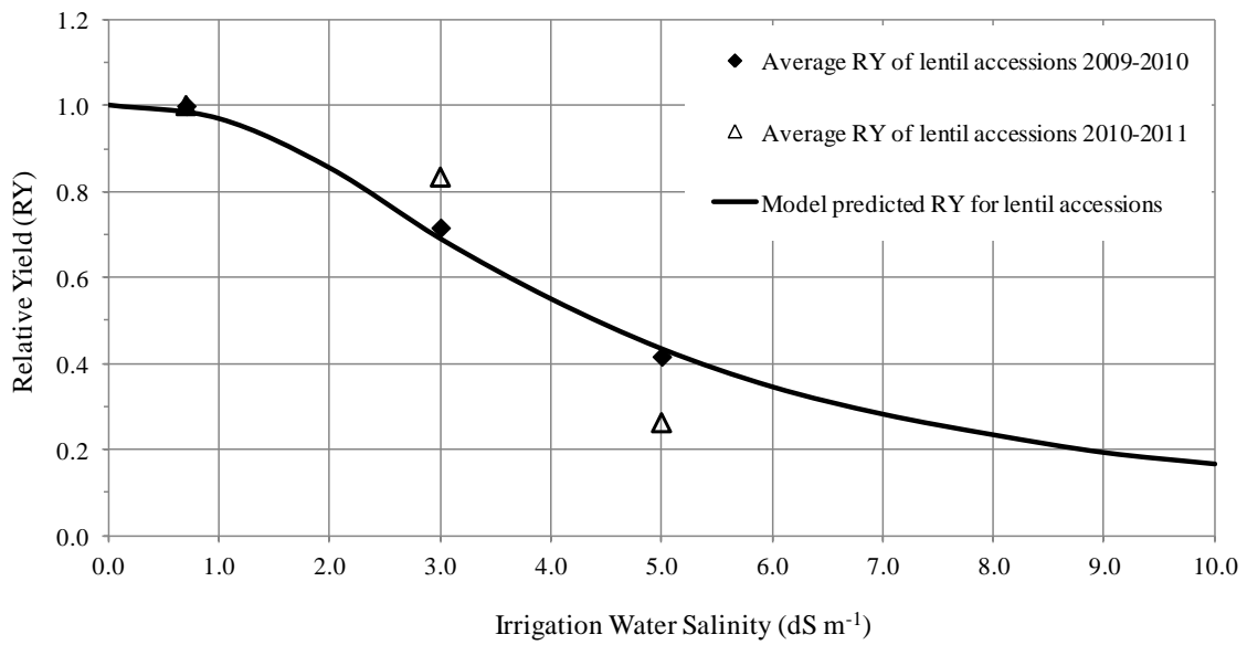
Figure 1. As predicted and validated by SALTMED model, decrease in relative grain yield of Lentil as affected by the incremental increase in irrigation water salinity up to 10 dS m -1
