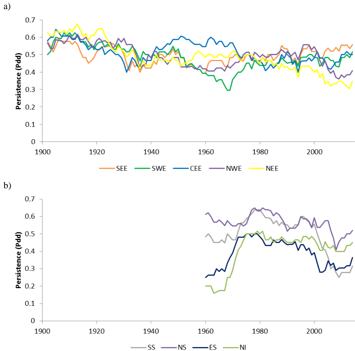
Figure 5 Dry-to-dry season persistence (Pdd) in the homogeneous rainfall regions of a) England and Wales, b) Scotland and Northern Ireland. All series are based on 30-year moving blocks with anomalies referenced to the 1961-1990 mean.
