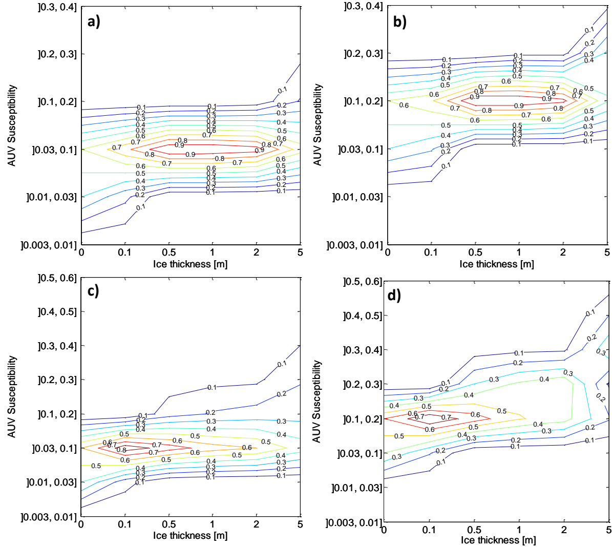
Figure 7. Variation of AUV Susceptibility with ice thickness. a) Nominal P(\text{loss}) instantiated at [0.03, 0.1], ice concentration set to 50%. b) Nominal P(\text{loss}) instantiated at [0.03, 0.1], ice concentration instantiated to 100%. c) Nominal P(\text{loss}) instantiated at [0.1, 0.2], ice concentration set to 50%. d) Nominal P(\text{loss}) instantiated at [0.1, 0.2], ice concentration set to 100%.
