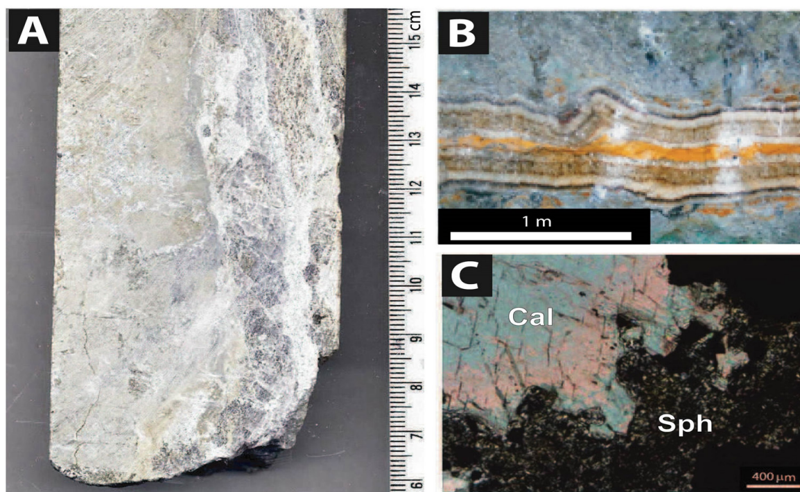
Figure 5 (A) Core sample showing epithermal vein of calcite (white) and fluorite (purple gray) cutting the skarn assemblage from the Santa María deposit (sample VW-158 AB). (B) Epithermal vein inside the Santa María mine, where several generations of growth are exhibited. (C) Photomicrograph of the sphalerite crystals in calcite vein (sample V-129-G, transmitted light, plane polarized light). Cal: calcite; Sph: sphalerite.
