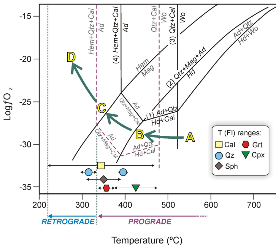
Figure 12 Temperature vs. O_2 fugacity diagram (Ca-Fe-Si-C-O-H system at 500 kbar; after Bowman 1998) showing suggested general paths for prograde (A, B, and C) and retrograde (D) stages of formation of the Velardeña skarns. Dashed lines: univariant curves at f(CO_2) of 1.5 MPa; solid lines: univariant curves at f(CO_2) of 6 MPa. Mineral abbreviations: Ad: andradite; Cal: calcite; Cpx: clinopyroxene (diopside); Grt: garnet (andradite); Hem: hematite; Hd: hedenbergite; Mag: magnetite; Qz: quartz; Sph: sphalerite; Wo: wollastonite.
