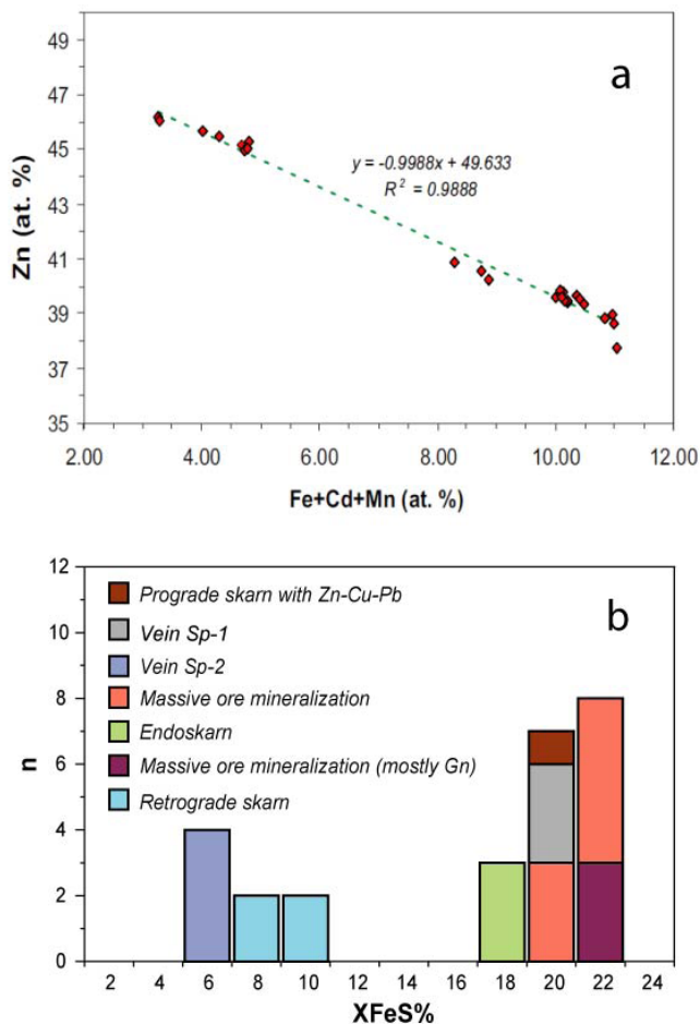
Figure 8 Composition diagrams of all sphalerite crystals (n = 67, electron microprobe data) from the Velardeña skarns and veins. (a) Zn vs. Fe + Cd + Mn plot, where 2 sphalerite types are plotted. (b) Histogram of iron contents, in X% FeS.
