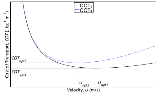
(d) Impact of halving equivalent spheroid efficiency (doubling propulsion power) on an individual's cost of transport.
