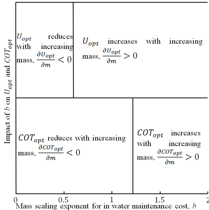
Figure 4. Impact of mass scaling exponent for the in water maintenance power requirements (for turbulent flow)
