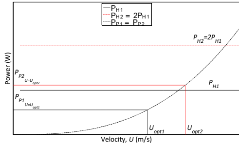
(a) Impact of doubling in-water maintenance cost on an individual's power requirements.
