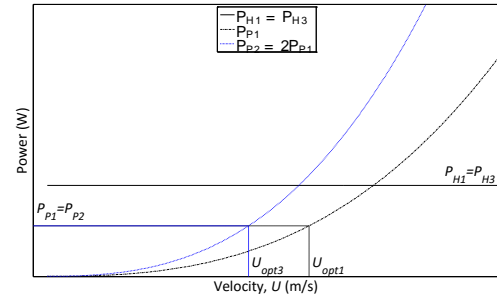
(b) Impact of halving equivalent spheroid efficiency (doubling propulsion power) over the speed range on an individual's power requirements.
