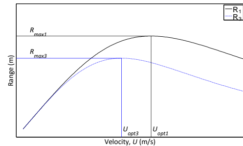
(f) Impact of halving equivalent spheroid efficiency (doubling propulsion power) on an individual's range.
