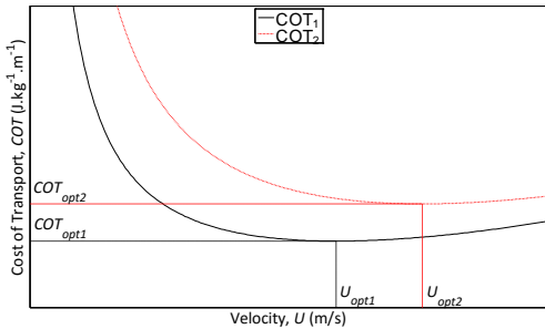
(c) Impact of doubling in-water maintenance cost on an individual's cost of transport.
