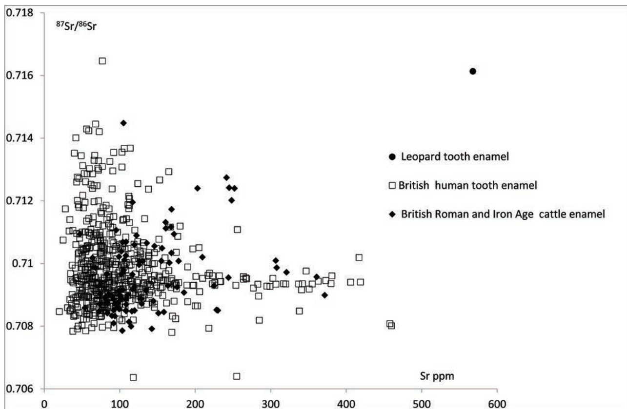
Figure 6: A comparison of the strontium isotope composition (y-axis) and strontium concentration (x-axis) from the enamel of the leopard tooth (PLYMG.2013.187) along with archaeological British data sets for human enamel (Evans, Chenery & Montgomery, 2012) and for cattle from southern England (Minniti et al., 2014).
