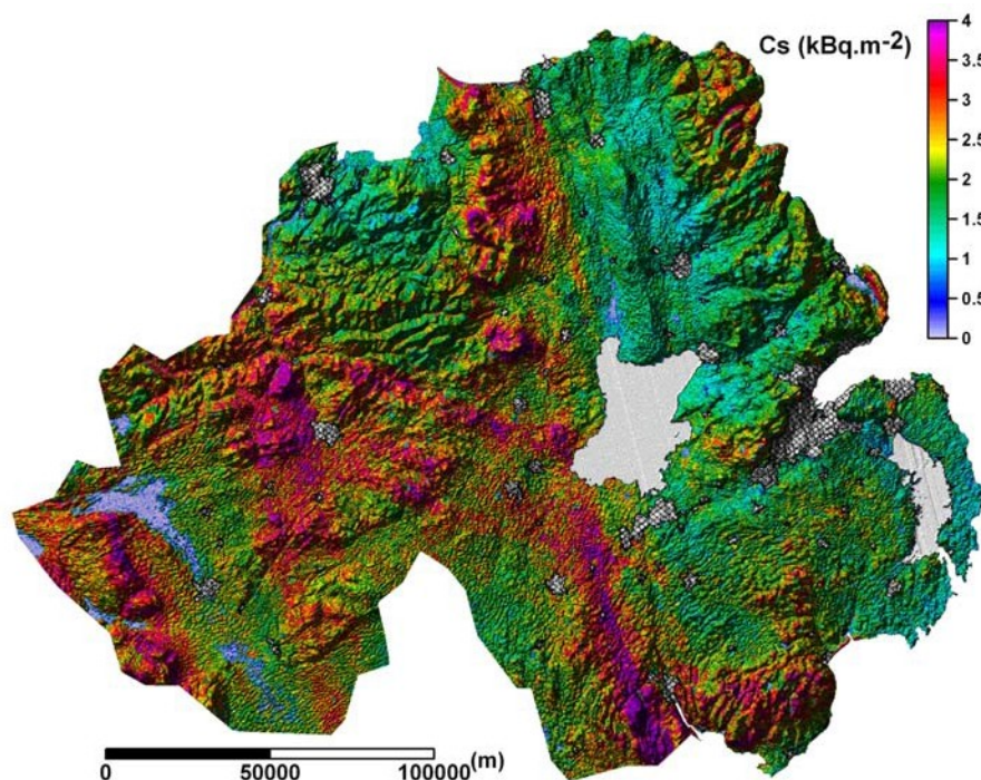
Figure 1. The ^{137}\text{Cs} distribution obtained from the Tellus survey of Northern Ireland. A continuous colour image derived from 100 \times 100 grid cells is shown draped on a base DTM. The distribution is cut to the coast. Centres of population ( >1000 people) are shown shaded with cross-hatch.
