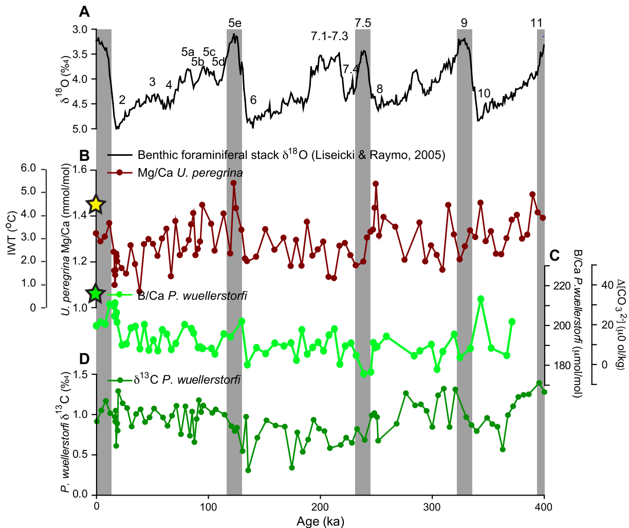
Fig. 4. Compilation of AAIW proxy records from DSDP593 A: benthic foraminiferal \delta^{18}\text{O} LR04 stack (black; Lisiecki and Raymo, 2005), B: \text{Mg}/\text{Ca}_{U. peregrina} (maroon), calculated as IWT according to Elderfield et al. (2010), C: \text{B}/\text{Ca}_{P. wuellerstorfi} (light green), calculated as \Delta[\text{CO}_3^{2-}] according to Rae et al. (2011), D: and \delta^{13}\text{C}_{P. wuellerstorfi} (forest green). (For interpretation of the references to color in this figure, the reader is referred to the web version of this article.)
