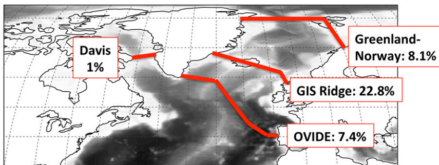
FIG. 6. Intrinsic-to-total LF variance ratio R from AMOC_{\sigma_2} time series computed across four sections from our 1/12^\circ simulations. The shaded background shows topography.
