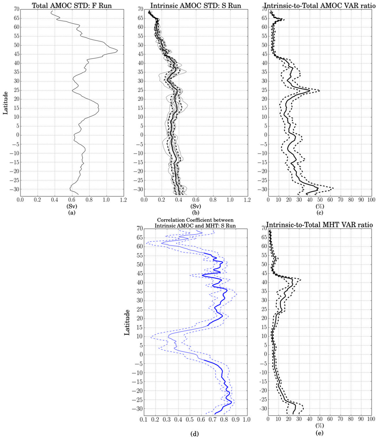
FIG. 5. (a) Total and (b) intrinsic interannual standard deviations of the AMOC σ 2 upper-cell northward limb transports at 1/4°, and (c) the ratio R of their variances. The nine successive 32-yr s_I estimates of intrinsic variability are shown in gray in (b). The solid and dashed black lines in (b) and (c) represent the averages and envelopes of the nine s_I estimates presented in section 2f. (d) Correlation between intrinsic interannual AMOC σ 2 and MHT variabilities at 1/4° over the nine successive 32-yr periods. Solid and dashed lines represent the mean and std dev of the correlation coefficient over the nine periods, respectively. Thick solid lines show where the correlations remain significant throughout the nine periods. (e) As in (c), but for the interannual MHT at 1/4° (envelope of M defined in section 2f). A nine-point moving average has been used to smooth these data.
