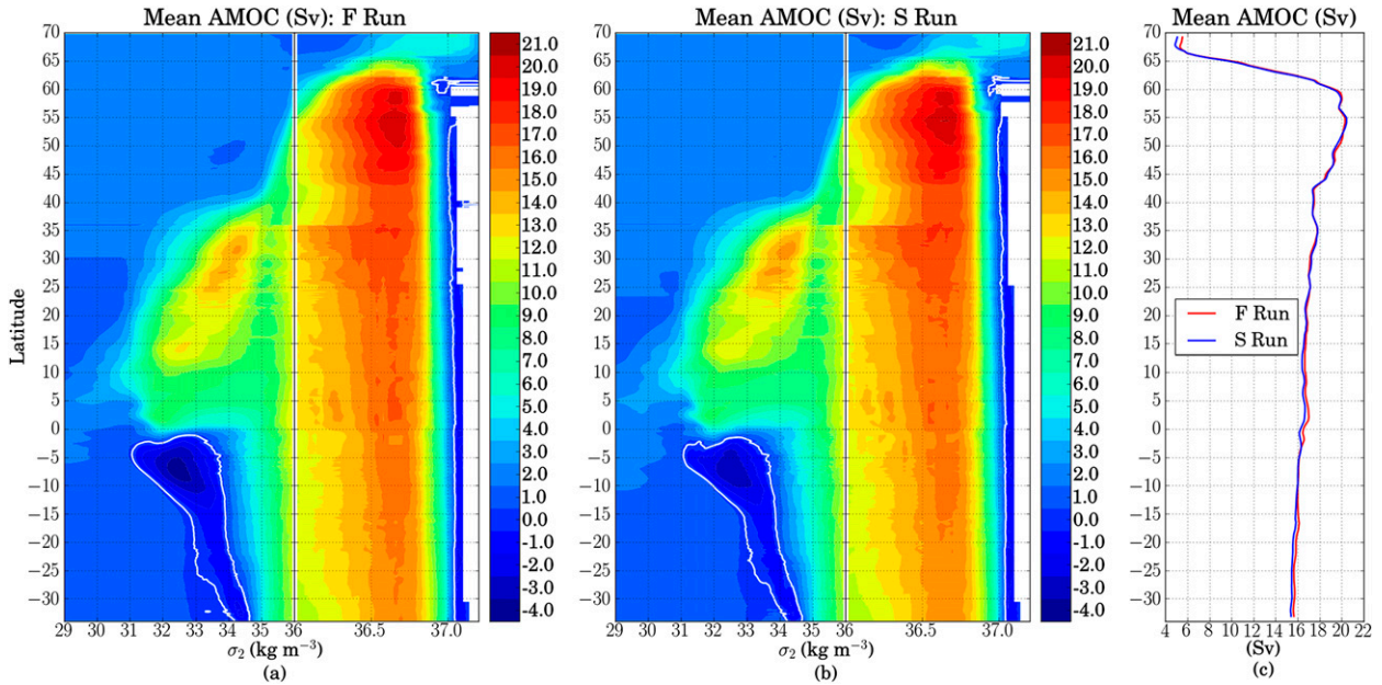
FIG. 1. Time-averaged \text{AMOC}_{\sigma_2} streamfunctions at 1/4^\circ (left) between 1976 and 2007 in the F run and (middle) between years 19–50 in the S run; zero contours are shown in white. (right) The time-averaged transport of the \text{AMOC}_{\sigma_2} upper-cell northward limb in both runs (i.e., maximum of AMOC in density coordinates; refer to section 2b); a nine-point boxcar filter has been used to smooth the data.
