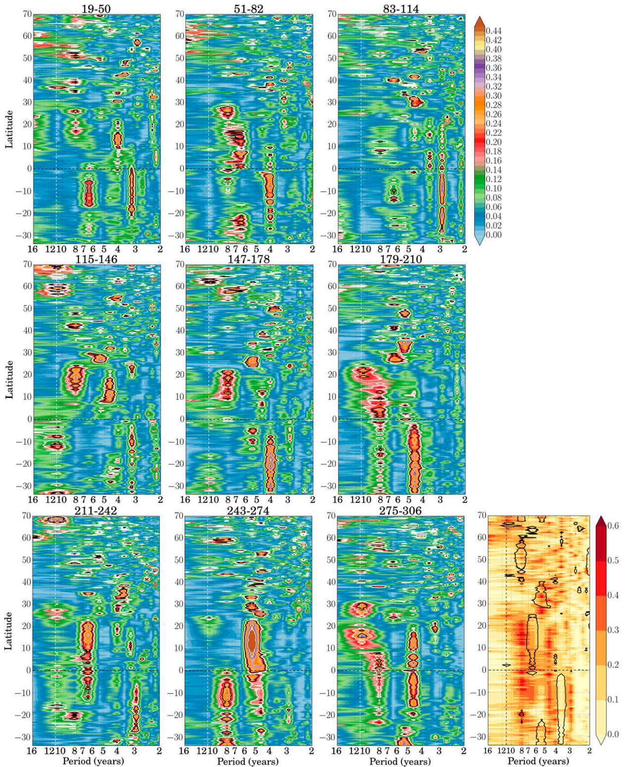
FIG. 9. (left) Frequency–latitude Fourier power spectra of the intrinsic AMOC_{\sigma_2} variability during the nine successive 32-yr periods of the 1/4^\circ S run. Spectra are normalized by the AMOC_{\sigma_2} interannual variance at each latitude. Black and white contour lines indicate 95% and 90% confidence levels, respectively. (bottom right) Probability that these intrinsic variability peaks are significant at 90% over the nine periods (color, refer to section 4b); regions of the frequency–latitude plane where total variability spectral peaks in the fully forced 1/4^\circ F run are significant at 90% (black contours, refer to section 4c). Dashed white/black line shows the cutoff period of the Loess detrending operator.
