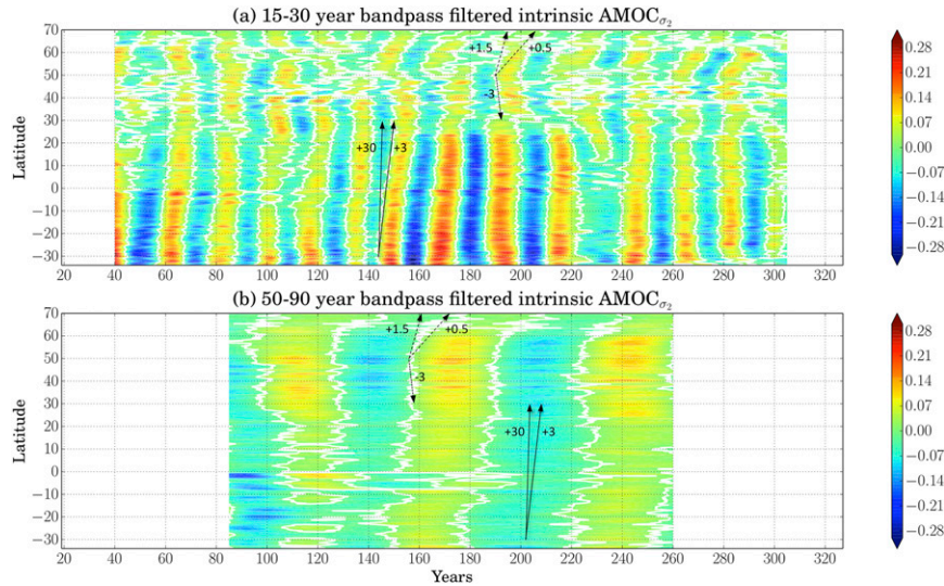
FIG. 10. Time–latitude plots of intrinsic AMOC_{\sigma_2} anomalies (Sv) during the 1/4^\circ S run, bandpass filtered (top) in the 15–30-yr band and (bottom) in the 50–90-yr band; initial and final parts of the time series are ignored because of the side effects of the Lanczos filters. Slanted lines and associated numbers indicate ranges of meridional phase speeds ( \text{cm s}^{-1} ) that dominate within selected latitude ranges; pluses and minuses correspond to northward and southward propagation, respectively.
