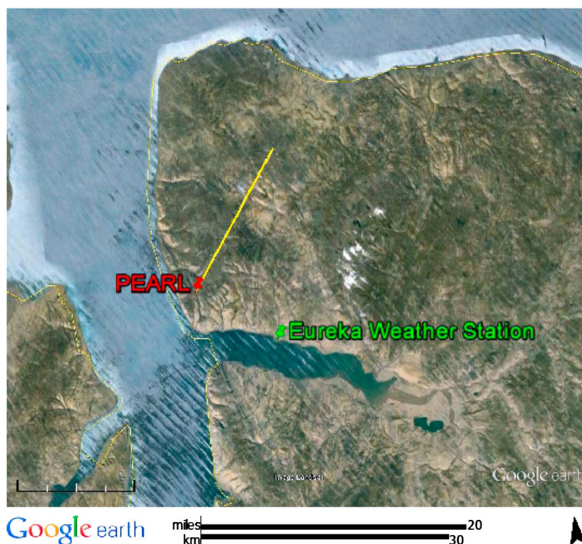
Figure 1. Locations of Eureka Weather Station and PEARL Ridge Lab (map data: Google earth). The yellow line (20 km in length) represents the viewing azimuth direction of MAX-DOAS measurements, which is 35° from true north.
