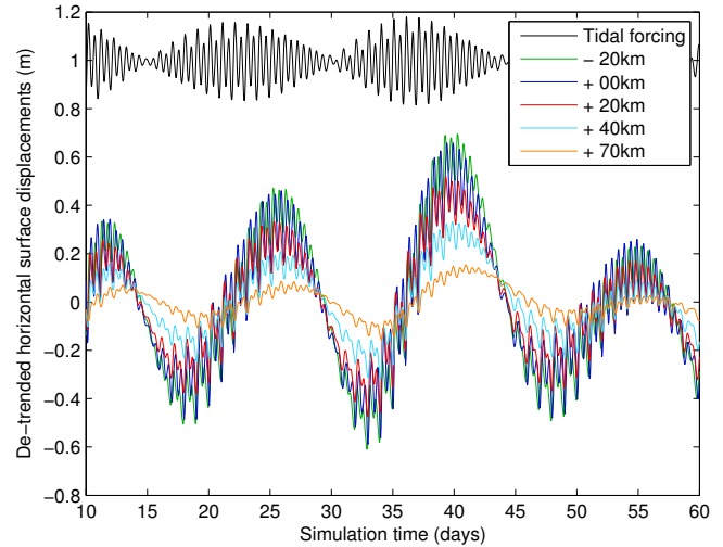
Figure 6. Modelled detrended horizontal surface displacements taken along the ice-stream medial line at 20 km downstream ( -20 km), at the grounding line ( +00 km) and distances of 20, 40 and 70 km upstream of the grounding line ( +20 , +40 and +70 km, respectively). The model was forced with \bar{N} = 105 kPa, K = 7 \times 10^9 m 2 d -1 , q = 10 , m = 3 , E = 4.8 GPa and \nu = 0.41 .
