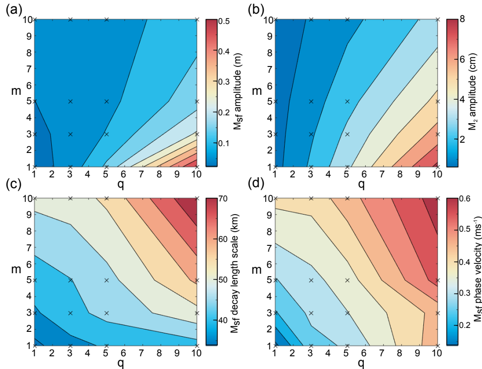
Figure 8. Response of M_{sf} amplitude (a), M_2 amplitude (b), M_{sf} decay length scale (c) and M_{sf} phase velocity (d) to choice of stress exponent ( m ) and hydrological exponent ( q ). Crosses indicate model simulations. M_{sf} and M_2 amplitudes were taken at 10 km upstream from the grounding line.
