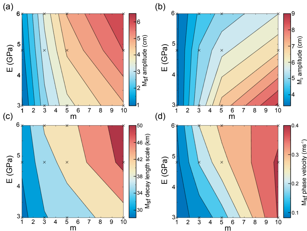
Figure 4. Modelled M_{sf} and M_2 tidal amplitudes 10 km upstream from the grounding line (a and b, respectively), and M_{sf} decay length scales and phase velocities (c and d, respectively) as a function of the basal sliding law stress exponent m and the elastic Young's modulus ( E ) of ice. Here the potential effects of subglacial water pressure variations in response to tides on sliding were not included, i.e. in the sliding law (Eq. 8), q = 0 . Crosses indicate model simulations. The contour plot is based on interpolation of model results. M_{sf} and M_2 amplitudes were taken at 10 km upstream from the grounding line.
