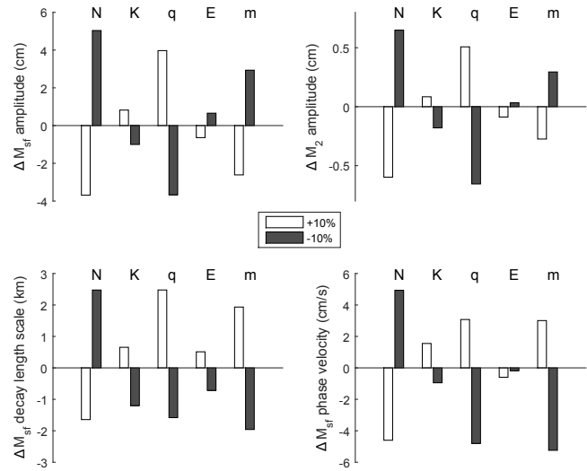
Figure 7. Sensitivity analysis of model parameters ( N , K , q , E and m ), showing change in M_{sf} and M_2 amplitudes (a and b), M_{sf} decay length scale (c) and M_{sf} phase velocity (d) for +10\% (white bar) and -10\% (grey bar) changes in each parameter. Model outputs were compared to the simulation presented in Fig. 6 and all other parameters were kept at the values defined in that plot.
