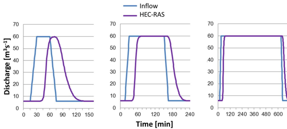
Figure 17.15 Illustration of the inflow and the simulated outflow hydrographs for a flow change rate of 1:10 and a upsurge duration of 30 minutes (left), 120 minutes (centre) and 600 minutes (right) (Auer, 2012).
