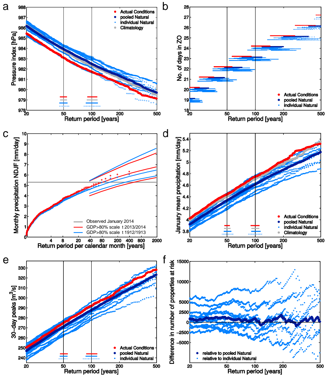
409 Figure 5: Return periods for a modelled January pressure index (each dot represents an ensemble 410 member) with 5-95% confidence intervals for 1-in-50-year events and 1-in-100-year events in Actual 411 Conditions estimated by resampling the distribution 100 times, represented as horizontal lines. Red 412 represents Actual Conditions simulations, grey a similar ensemble but for 1986-2011 (the model 413 climatology), dark blue the pooled Natural simulations, and light blue individual Natural (sub-) 414 ensembles, with solid circles for the 6 of the 11 Natural ensembles with around 15,000 simulations, and 415 empty circles for the other 5 with around 7,000 simulations. Only four 5-95% confidence intervals for 1- 416 in-50-year events and 1-in-100-year events (red: Actual Conditions, grey: Climatology, light blue: Natural 417 ensembles with around 15,000 ensemble members and dashed light blue: Natural ensembles with 418 around 7,000 simulations) are shown because the confidence intervals represent only the sampling 419 uncertainty, not the uncertainty in the estimation of the model simulations. b as a but modelled
