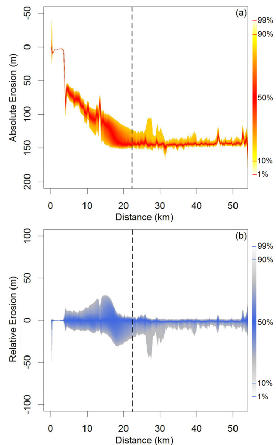
Figure 5. Simulated absolute change in coastline position (a) from 2010 to 2100 predicted using an ensemble of future wave climates. Relative change in coastline position (b) , as referenced to the baseline for each member of the ensemble. The range of colours in each plot represents the ensemble percentiles as given on the right of the figures. The black dashed line represents the divide between the northern region (to the left) and the southern region (to the right) as defined in the text.
