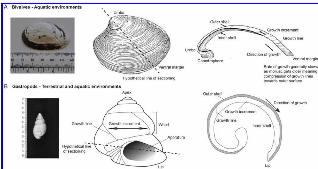
Figure 2 Mollusc sampling protocols: top left, modern freshwater bivalve specimen of Unio sp. from Çatalhöyük, Turkey (Bar-Yosef Mayer et al. 2012) and bottom left, terrestrial gastropod Limicolaria kambeul chudeau Germain from margins of Lake Tilo, Ethiopia (Leng et al. 1998) showing sampled cross sections (i.e. holes along the/whorl) for \delta^{18}\text{O} analysis. Drawings represent morphology of a bivalve (top centre and top left) and gastropod (top centre and top left) shell (modified from Prendergast and Stevens 2013).
