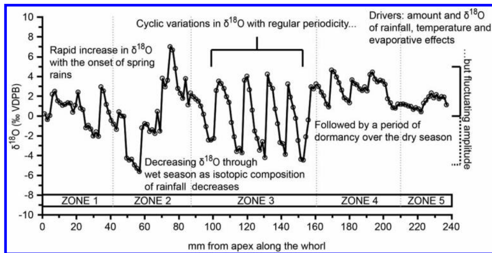
Figure 3 Annotated \delta^{18}\text{O} profile (plotted at intervals of 1.5 mm) from a modern land snail Limicolaria kameul chudeau Germain collected from the margins of Lake Tilo, Ethiopian Rift Valley near Awassa (Leng et al. 1998), showing annual climate cycles from the shell \delta^{18}\text{O} . Ten cycles are present spanning the lifetime of the individual shell.
