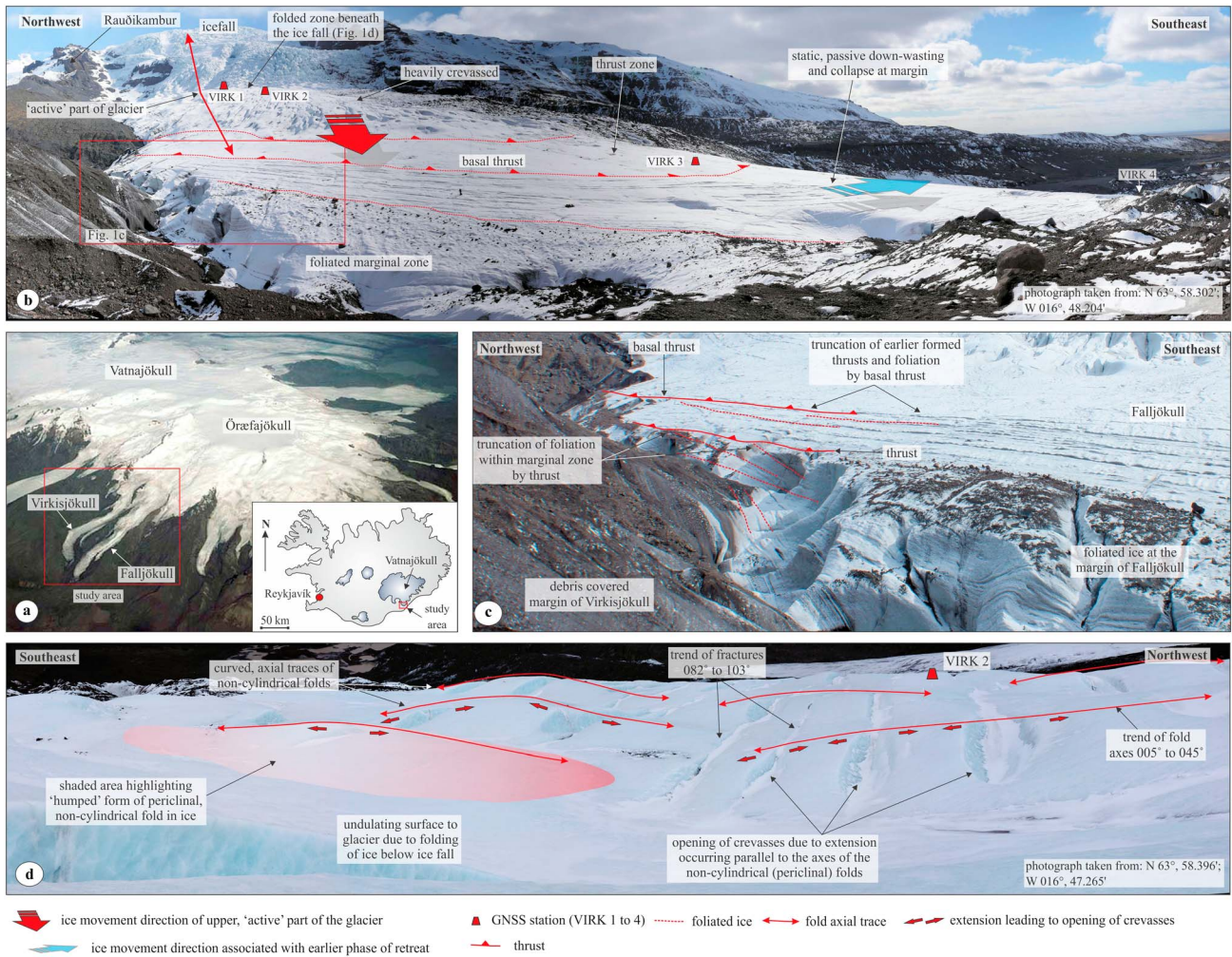
Figure 1. (a) Oblique air photograph of Örafajökull showing the location of the twin outlet glaciers Virkisjökull and Falljökull (image from LineLeak.com). Inset—Simplified map of Iceland showing the location of the study area on the southern side of the Vatnajökull ice cap. (b) Photograph of Falljökull showing the main glaciological deformation structures, ice movement directions in the upper and lower parts of the glacier, and the location of four GNSS stations (VIRK 1 to 4). (c) Photograph of the northwestern margin of Falljökull showing the basal thrust cutting earlier formed thrusts and zone of steeply inclined foliated ice. (d) Photograph showing the undulating surface of the glacier immediately below the icefall reflecting the periclinal folding of the ice.
