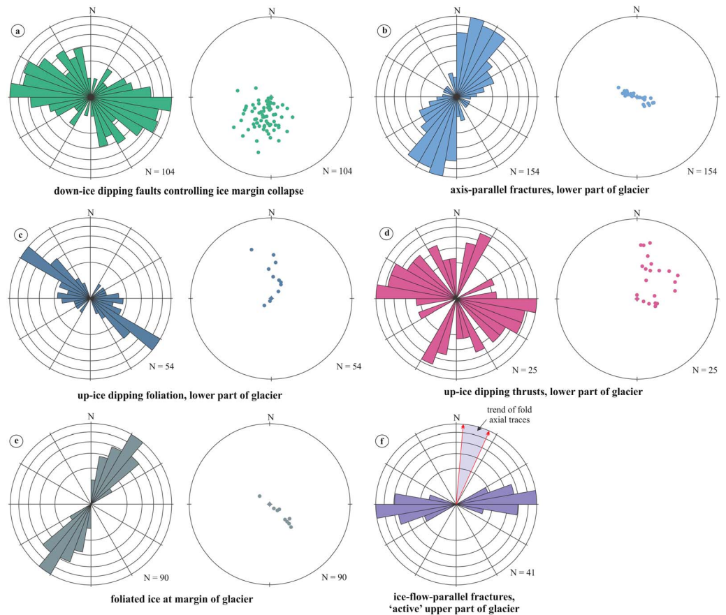
Figure 3. Structural data plotted on a series of rose diagrams (strike and dip azimuth): (a) Down-ice dipping faults; (b) axis-parallel fractures, lower part of the glacier; (c) up-ice dipping foliation, lower part of glacier; (d) up-ice dipping thrusts, lower part of the glacier; (e) foliation at margin of glacier; and (f) trend of ice flow-parallel fractures and fold axes in active upper part of the glacier.
