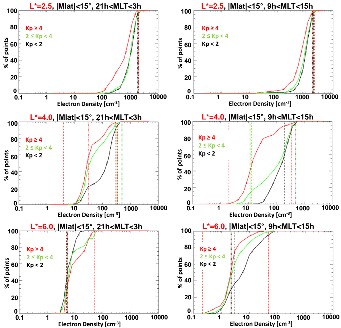
Figure 2. Electron plasma density (cm -3 ) resulting from CRRES measurements versus percentage of cumulated points for three L^* values ( L^* = 2.5 on top, L^* = 4.0 in the middle and L^* = 6.0 at the bottom), for two MLT intervals (around midnight on the left and around noon on the right). On each plot, three magnetic activities are represented: quiet (in black), moderate (in green) and active (in red). Results from the GCPM, Sheeley and Carpenter models are also represented in dashed lines, dash-dot lines and dash-dot-dot-dot lines, respectively.
