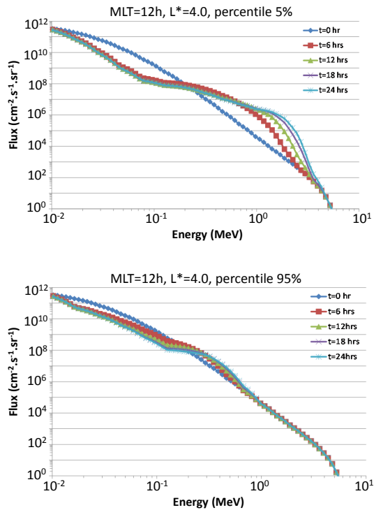
Figure 8. Time evolution of electron flux due to chorus and hiss waves at MLT = 12 h for L^* = 4.0 using extreme electron plasma density values: percentile 5 % on top (low density) and percentile 95 % on bottom (high density). The flux is shown at interval of 6 h.
