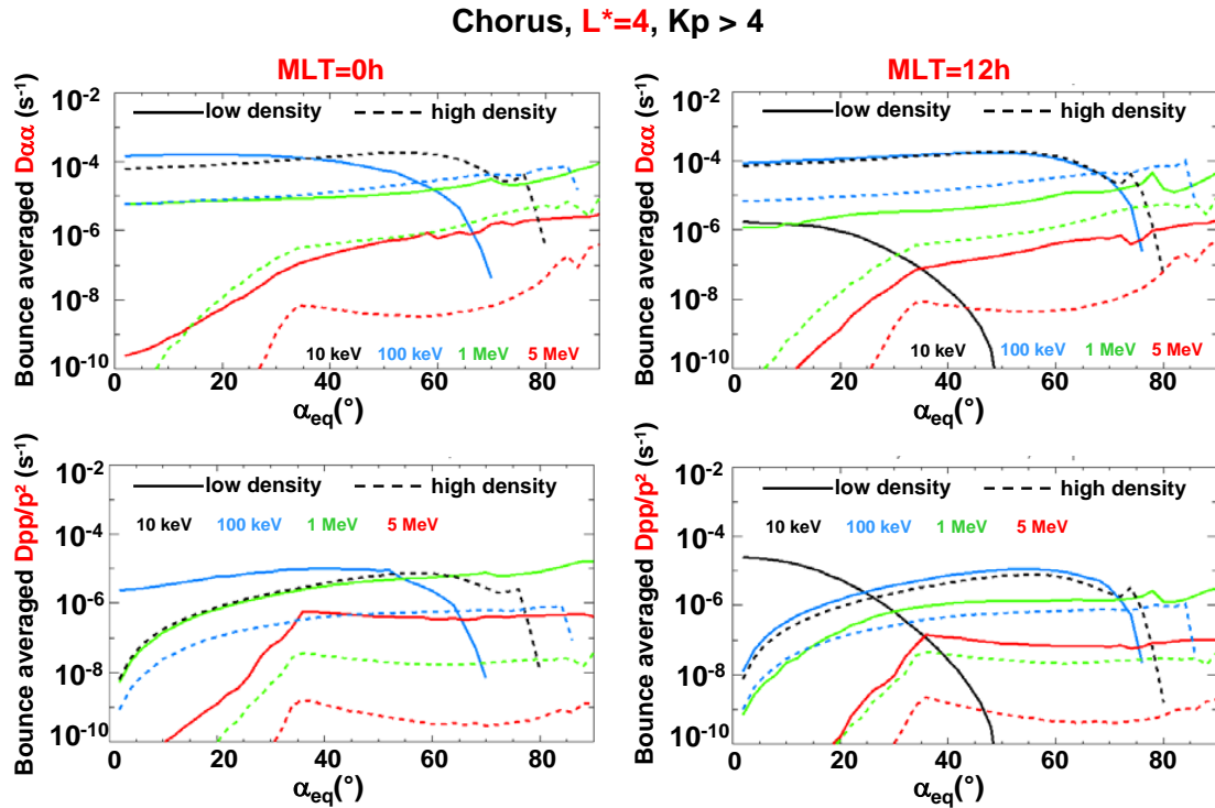
Figure 3. Bounce-averaged pitch angle (top) and energy (bottom) diffusion rates ( s^{-1} ) for chorus using WAPI code for 4 energies, 0.01 MeV (black), 0.1 MeV (blue), 1 MeV (green) for and 5 MeV (red) L^* = 4 and for MLT = 0 h on the left and MLT = 12 h on the right for active magnetic activity ( K_p > 4 ) and for two different plasma densities: 5th percentile in solid lines and 95th percentile in dashed lines.
