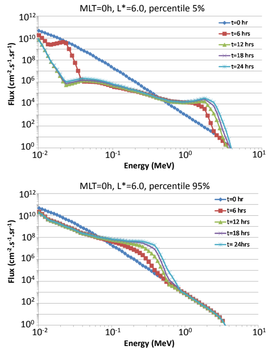
Figure 7. Time evolution of electron flux due to chorus waves at MLT = 0 h for L^* = 6.0 using extreme electron plasma density values: percentile 5 % on top (low density) and percentile 95 % on bottom (high density). The flux is shown at interval of 6 h.
