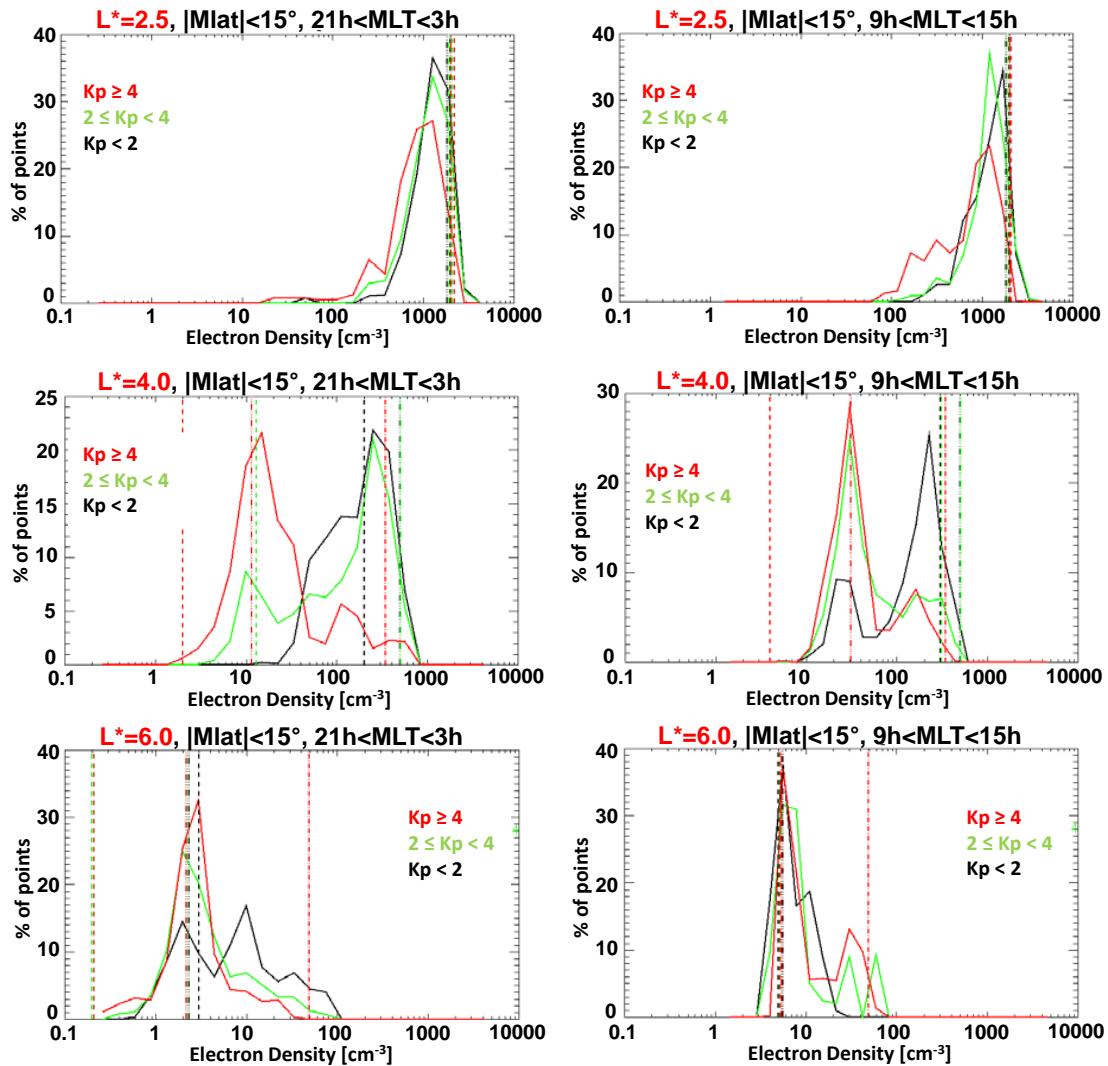
Figure 1. Electron plasma density ( \text{cm}^{-3} ) resulting from CRRES measurements versus percentage of points for three L^* values ( L^* = 2.5 on top, L^* = 4.0 in the middle and L^* = 6.0 at the bottom), for two MLT intervals (around midnight on the left and around noon on the right). On each plot, three magnetic activities are represented: quiet (in black), moderate (in green) and active (in red). Results from the GCPM, Sheeley and Carpenter models are also represented in dashed lines, dash-dot lines and dash-dot-dot-dot lines respectively.
