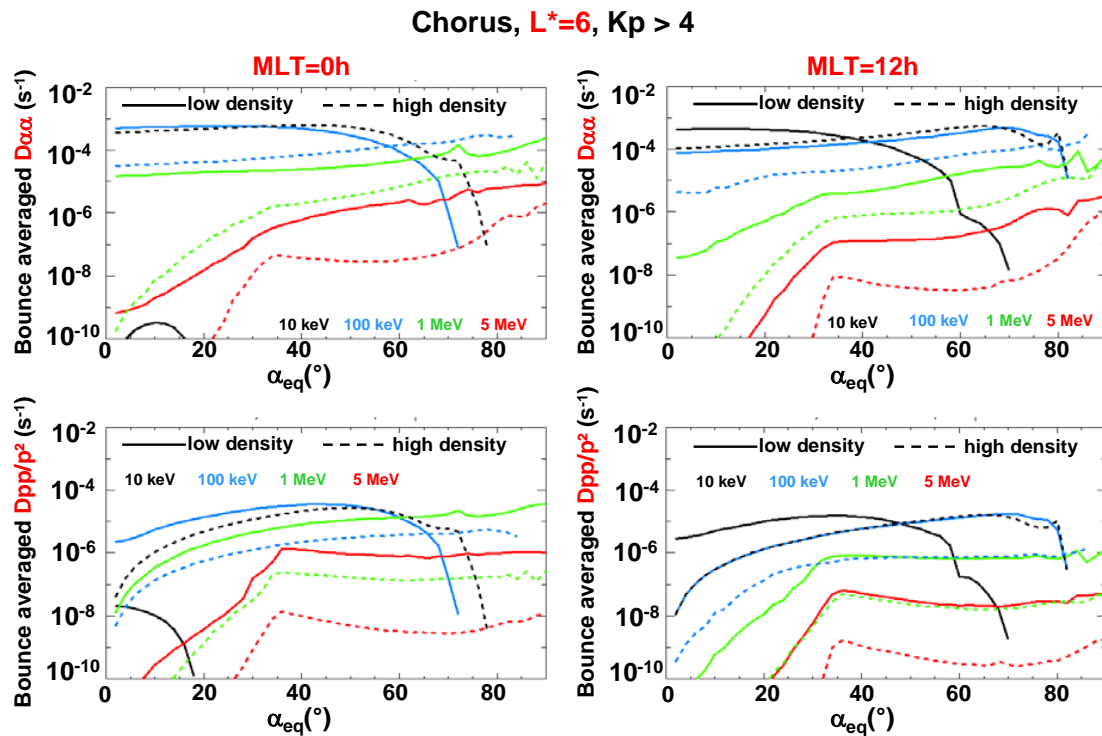
Figure 4. Bounce-averaged pitch angle (top) and energy (bottom) diffusion rates ( s^{-1} ) for chorus using WAPI code for 4 energies, 0.01 MeV (black), 0.1 MeV (blue), 1 MeV (green) for and 5 MeV (red) L^* = 6 and for MLT = 0 h on the left and MLT = 12 h on the right for active magnetic activity ( K_p > 4 ) and for two different plasma densities: 5th percentile in solid lines and 95th percentile in dashed lines.
