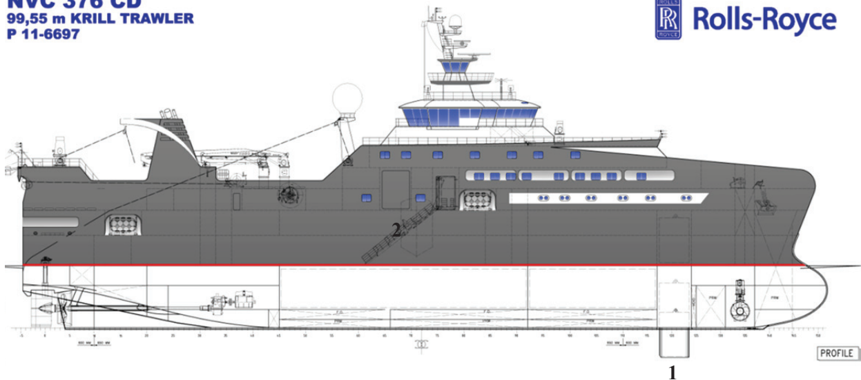
Figure 1: The new krill vessel with an instrument drop keel (1) and a hangar for operation of ROV and oceanographic and biological sampling gears (2). The vessel is 99 m long and has diesel electric propulsion.
