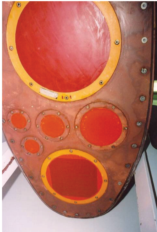
Figure 2: The tip of the drop keel with six acoustic frequencies (from RV G.O. Sars ). The intention is that the tip can be demounted and replaced by another module with tailored sensors in accordance with cruise objectives.
