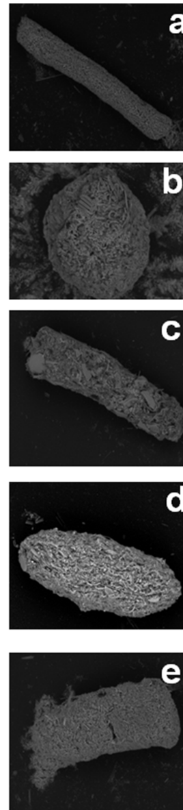
Figure 2. Scanning electron micrographs of the different FP types collected in the sediment traps: (a) cylindrical, (b) round, (c) ellipsoidal, (d) ovoid, (e) tabular.
