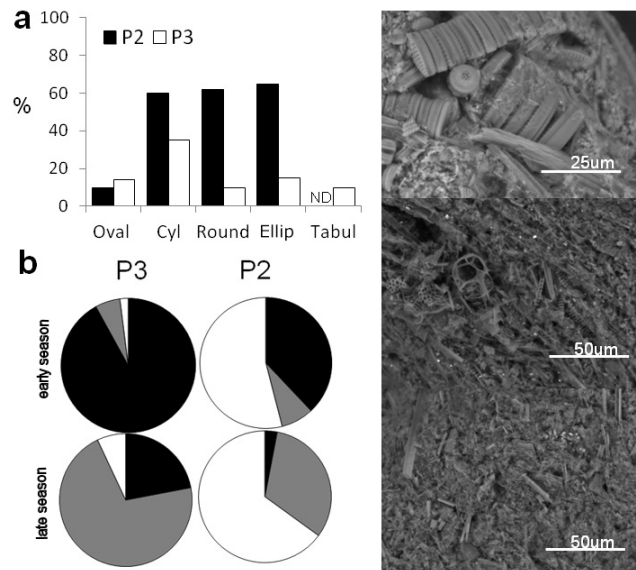
Figure 5. Left: (a) percentage of FP with evidence of degradation (i.e. fragmented and/or with the peritrophic membrane partially broken) at P3 and P2; (b) percentage of FP within sediment trap samples from early season (upper) and late season (lower) at P3 and P2, presenting mainly a content of intact diatoms (grey), fragmented diatoms (black) and reworked material (white). Right: scanning electron micrographs showing the diversity of FPs within sediment trap material.
