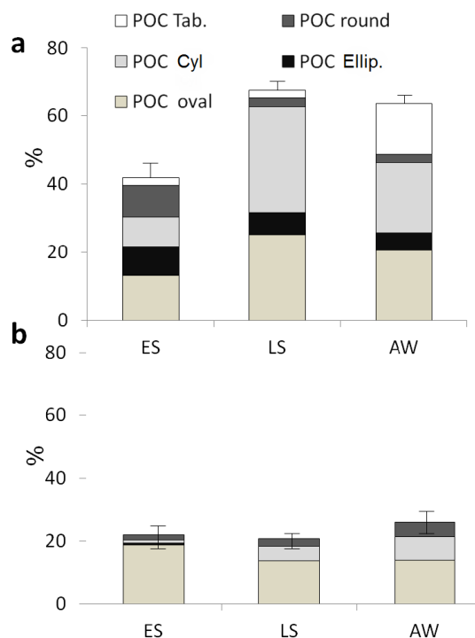
Figure 7. %FPC to total POC of each FP types during early season (ES), late season (LS) and autumn–winter (AW) at P3 (upper) and P2 (lower). Values were averaged over the period 2008–2011. Note: cylindrical attributable to krill and large copepods, tabular to salps, ovoidal to small copepods and pteropods, round to small copepods and amphipods, and ellipsoidal to larvaceans. Error bars indicate the standard error of the mean.
