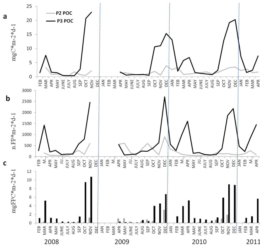
Figure 3. Interannual variability (2008–2011) of (a) POC ( \text{mg C m}^{-2} \text{d}^{-1} ), (b) FP ( \text{n. FP m}^{-2} \text{d}^{-1} ), (c) FPC ( \text{mg FPC m}^{-2} \text{d}^{-1} ) at P3 (black) and P2 (grey).
