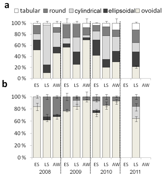
Figure 4. Percentage contribution of different FP types to total FP community between 2008 and 2011 at P3 (upper) and P2 (lower). Data is grouped according to season: ES stands for early season, LS for late season, AW for autumn–winter. Note: cylindrical attributable to krill and large copepods, tabular to salps, ovoidal to small copepods and pteropods, round to small copepods and amphipods, and ellipsoidal to larvaceans. Error bars indicate the standard error of the mean.
