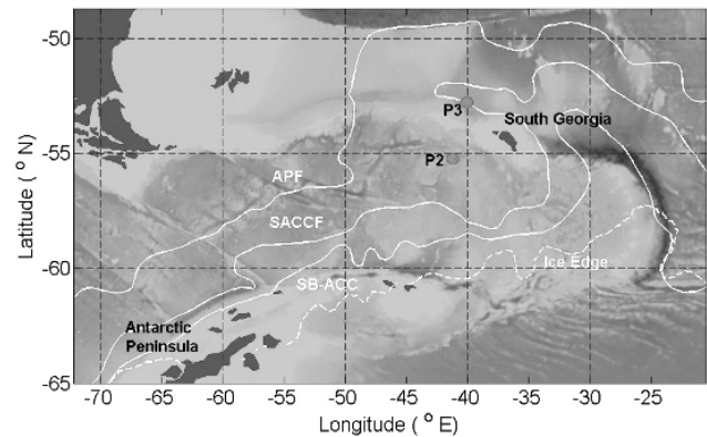
Figure 1. Map of study area in the Southern Ocean showing the locations of P3 and P2. APF stands for the Antarctic Polar Front, SACCF for Southern Antarctic Circumpolar Current Front and SB-ACC Southern Boundary of Antarctic Circumpolar Current.
