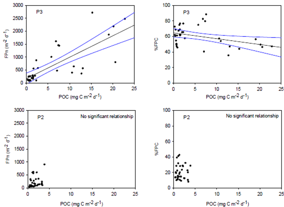
Figure 6. Relationship between POC ( \text{mg C m}^{-2} \text{d}^{-1} ) and FPn ( \text{m}^{-2} \text{d}^{-1} , left), on the one hand, and %FPC (right), on the other hand, for P2 and P3. Solid lines show fitted regressions with 95 % confidence intervals.
