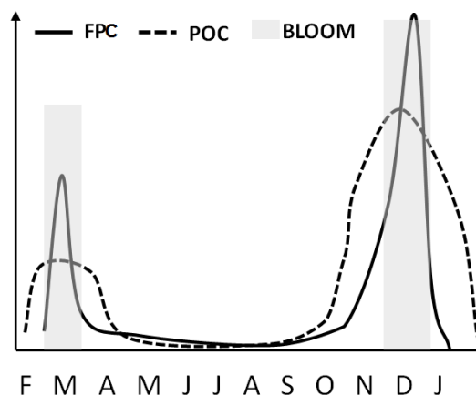
Figure 8. Schematic diagram representing the recurrent trend of POC and FPC flux (from 2008 to 2011) in relation to the bloom periods at the P3 site.
