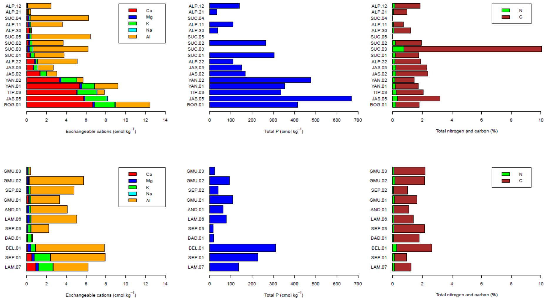
Fig S3. Topsoil (0-30 cm) properties by plot. Top panel presents data for Amazonian plots and bottom panel, Bornean plots. All plots are ordered in decreasing sum of bases ( \Sigma_B ) from bottom to top of plots. From left to right: mean concentrations of base cations (Ca, Mg, K, Na and Al in \text{cmol kg}^{-1} ); total P ( \text{mg kg}^{-1} ); total N and C(%).
