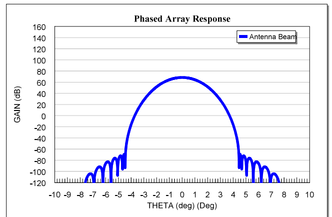
Fig. 8 75 by 75 Element, 0 dB Antenna Beam Profile
