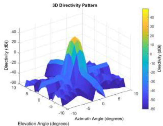
Fig. 4 Hexagonal Perimeter Beam Pattern
