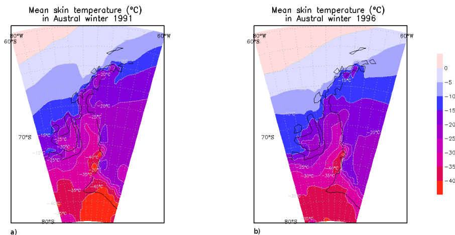
Figure 12. Mean skin temperature in winters 1991 (a) and 1996 (b) on the basis of ERAI reanalysis.
