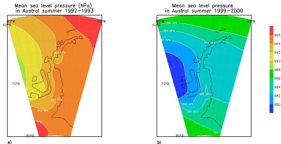
Figure 5. Mean sea level pressure (hPa) in austral summers 1992–1993 (a) and 1999–2000 (b) on the basis of ERAI reanalysis.
