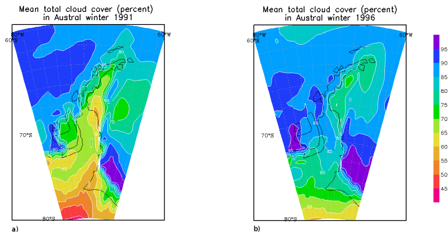
Figure 11. Mean cloud fraction in austral winters 1991 (a) and 1996 (b) on the basis of ERAI reanalysis.
