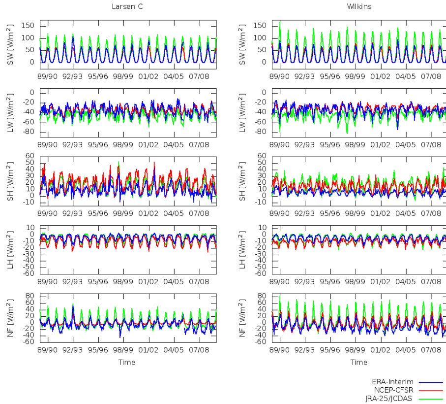
Figure 3. Time series of monthly mean surface energy fluxes on Larsen C and Wilkins ice shelves based on ERAI, CFSR and JRA reanalyses.
