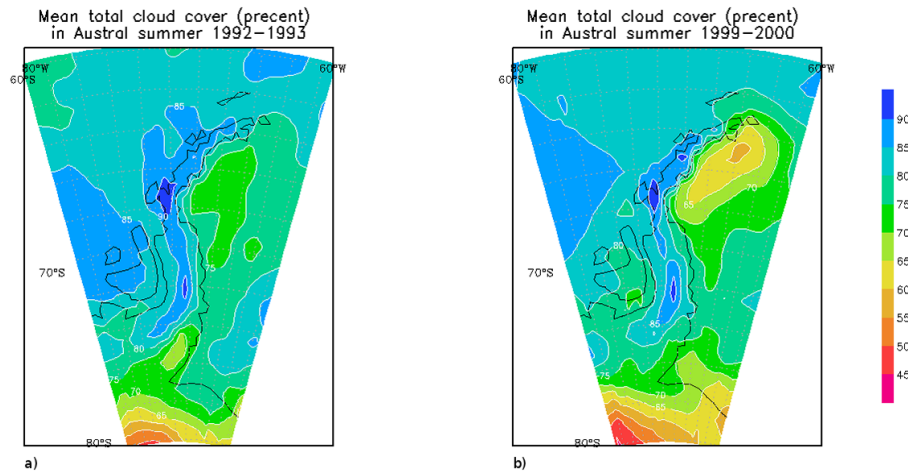
Figure 7. Mean cloud fraction in austral summers 1992–1993 (a) and 1999–2000 (b) on the basis of ERAI reanalysis.
