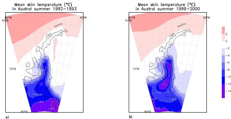
Figure 8. Mean skin temperature in austral summers 1992–1993 (a) and 1999–2000 (b) on the basis of ERAI reanalysis.
