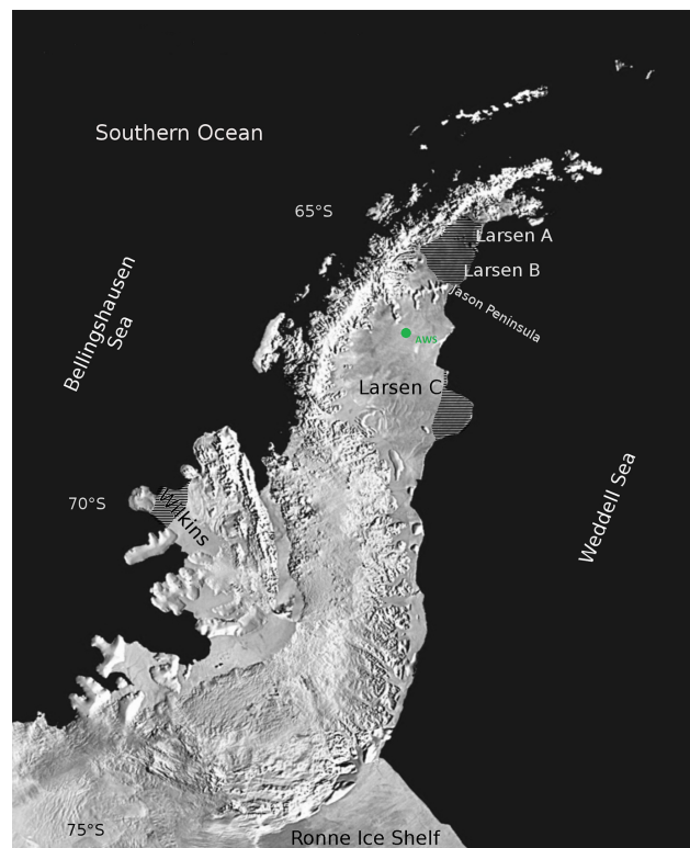
Figure 1. Antarctic Peninsula. Modified from NASA's Blue Marble data set (MODIS AVHRR). The disintegrated parts of Larsen and Wilkins ice shelves are marked as thin stripes, and the location of the automatic weather station used in this study is shown as a green circle.
