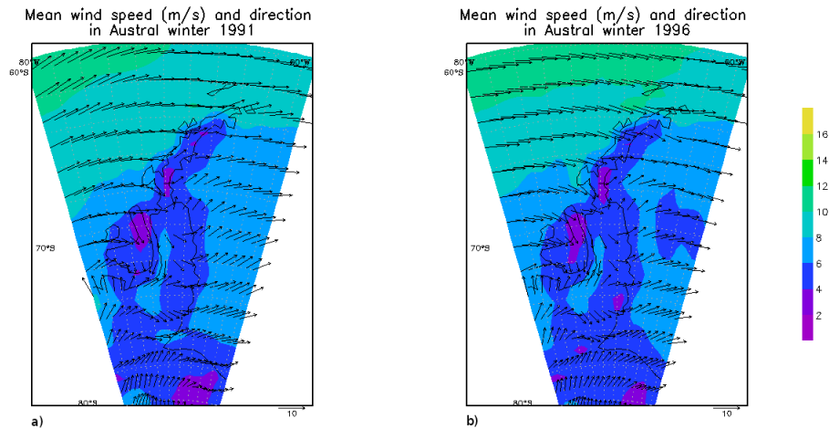
Figure 10. Mean wind speed and direction in winters 1991 (a) and 1996 (b) on the basis of ERAI reanalysis.
