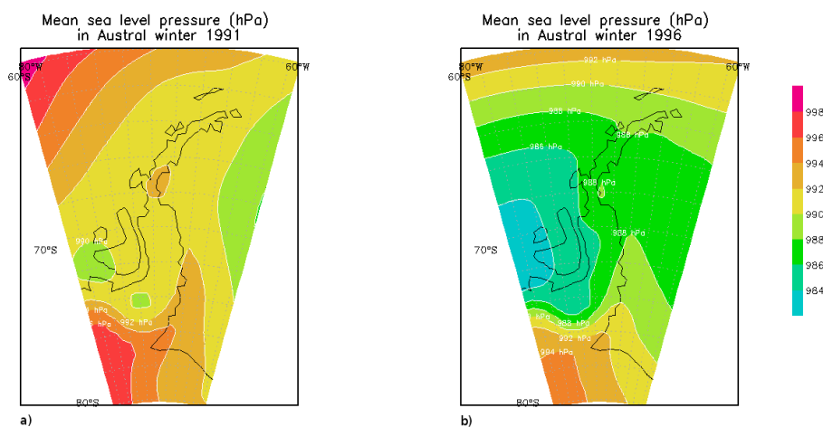
Figure 9. Mean sea level pressure in austral winters 1991 (a) and 1996 (b) on the basis of ERAI reanalysis.
