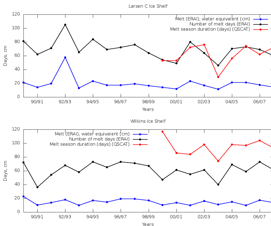
Figure 2. Mean summertime melting and number of melt days on Larsen C and Wilkins ice shelves calculated on the basis of ERAI reanalysis and retrieved from QSCAT observations by Barrand et al. (2013).
