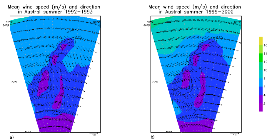
Figure 6. Mean wind speed ( \text{m s}^{-1} ) and direction in austral summers 1992–1993 (a) and 1999–2000 (b) on the basis of ERAI reanalysis.
