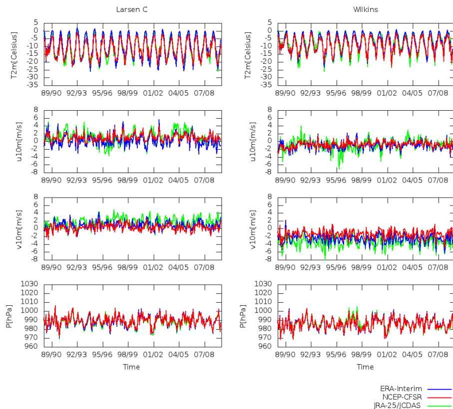
Figure 4. Time series of 2 m air temperature, 10 m wind speed and mean sea level pressure on Larsen C and Wilkins ice shelves on the basis of ERAI, CFSR and JRA reanalyses.
