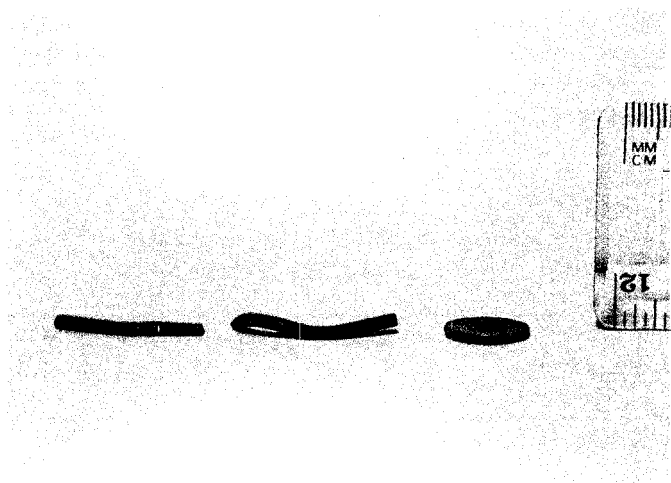
Fig. 1. SMA NiTi Rods and Disc were used in some of the candidate products, refer to Table 4. First, all NiTi 1-way actuators were trained and mechanically deformed, then inserted into the products for disassembly experiments.
