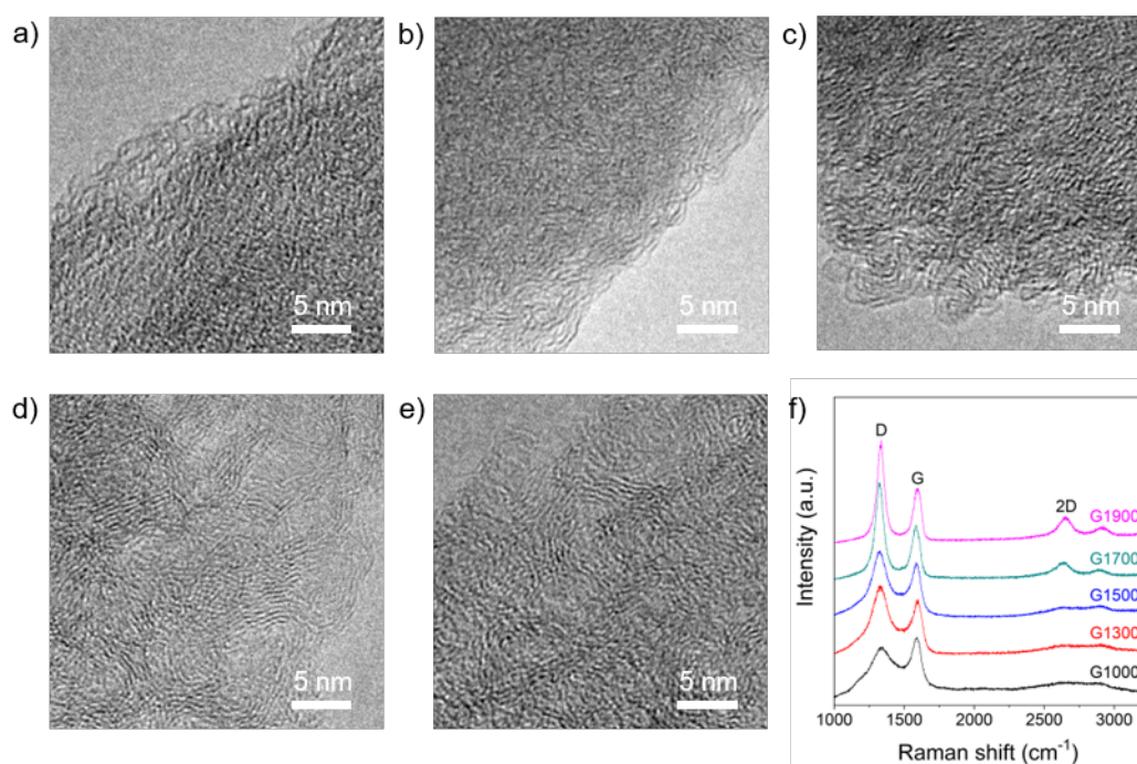
Figure 2. TEM images of a) G1000, b) G1300, c) G1500, d) G1700, and e) G1900; scale bars 5 nm; f) Raman spectra of G1000, G1300, G1500, G1700 and G1900, \lambda_{exc} = 633 nm.
