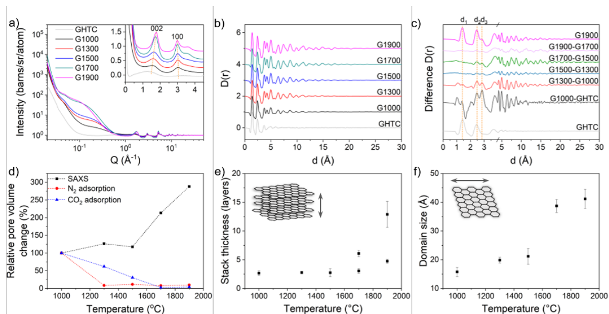
Figure 3. a) Structure factor ( S(Q) ), and b) PDF ( D(r) ) of the carbons before and after high temperature treatment. The SANS region was removed before Fourier transform to the PDF to remove pore-pore correlations; c) difference PDF between each temperature with the PDF of GHTC and G1900 included for reference; d) relative change in the pore volume probed by N_2 and CO_2 gas adsorption and the intensity of the Guinier plateau in the small angle region weighted by pore volume; e) stack thickness, and f) domain size of the graphitic regions derived from the width of the 002 and 100 peaks. Additional SAXS data and example model fits are shown in Figure S3.
