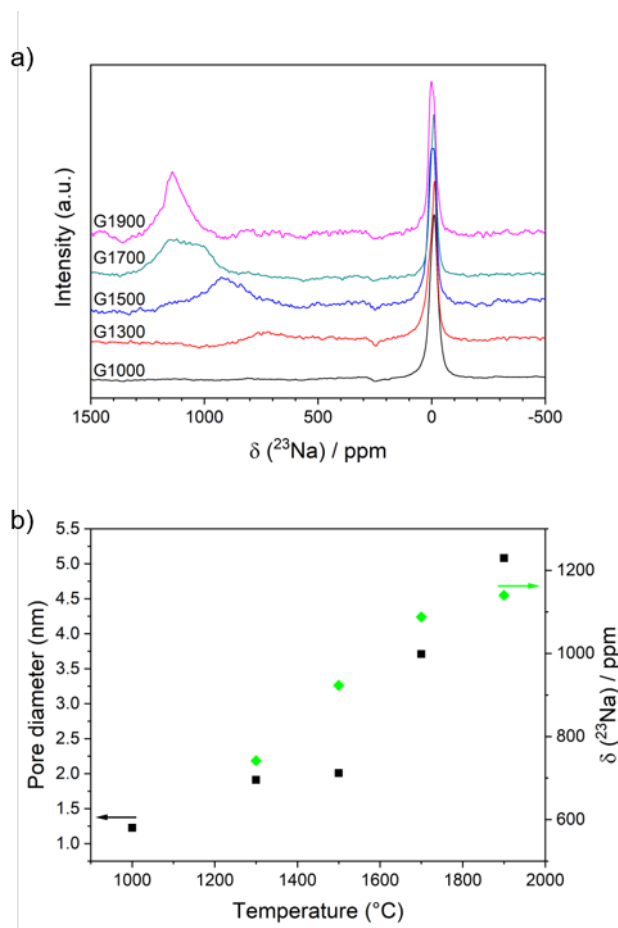
Figure 4. a) Ex situ ^{23}\text{Na} MAS NMR of G1000-G1900 after discharging to 5 mV, b) relationship between the pore diameter, quasi-metallic Na peak shift and sample pyrolysis temperature.
