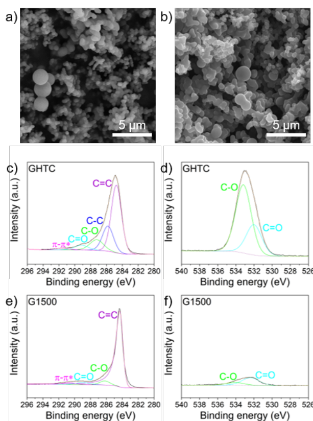
Figure 1. SEM images of a) GHTC and b) G1500; scale bars 5 \mu\text{m} ; core level c) C1s and d) O1s spectra for GHTC; core level e) C1s and f) O1s spectra for G1500.
