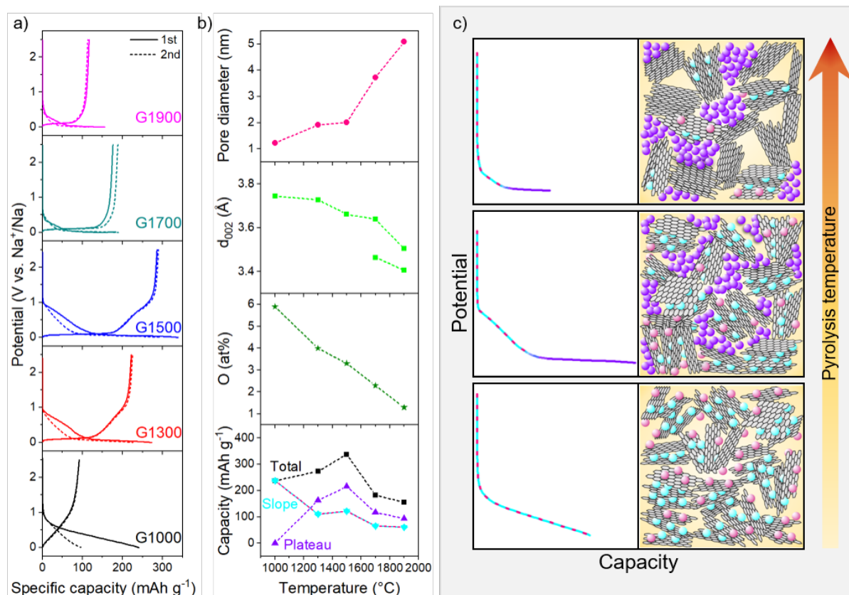
Figure 5. a) Galvanostatic charge/discharge profiles for G1000-G1900 in the first and second cycles; b) summary of the structural evolution of the hard carbons and capacity contributions with increasing pyrolysis temperature (lines are a guide for the eye only); c) schematic illustration of the proposed sodium storage mechanism; stack thickness and plane size are not to scale, and defects and curvature are not explicitly shown.
