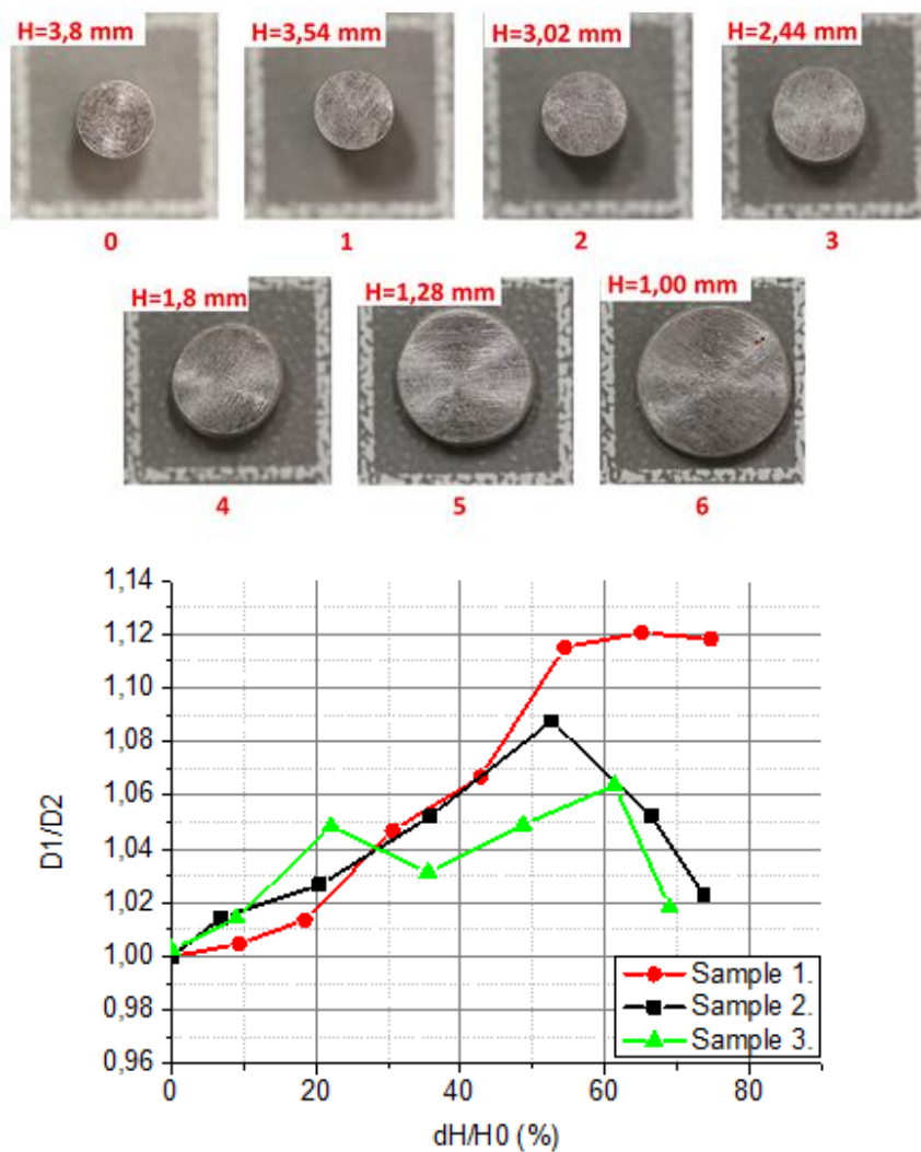
Figure 6. Results of multi-step compression test. Samples 1, 2 and 3 are parallel tests.
