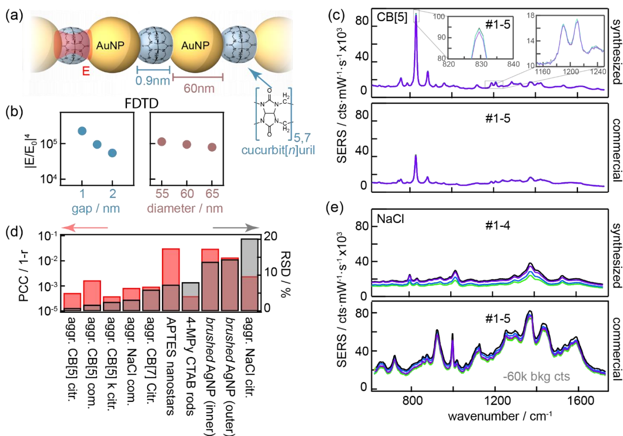
Figure 1: Reproducibility in SERS substrates, (a) Schematic representation of CB[5] aggregated AuNPs with 0.9 nm separation, (b) FDTD simulation of SERS enhancement as a function of gap size and AuNP size (calculated as E^2_{633nm} * E^2_{700nm} ). (c) SERS spectra comparison between homemade (top) vs commercial (bottom) AuNPs aggregated using CB[5], showing comparable reproducibility but lower counts for commercial AuNPs. Each spectrum represents another batch taken on a different day. (d) Comparison of the reproducibility for various SERS substrates using a Pearson correlation coefficient analysis and the relative standard deviation (RSD). (e) Salt-induced aggregation of both types of AuNP, showing larger spectral variance and an increased background for commercial particles.
