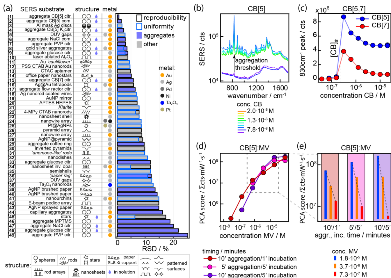
Figure 2: Factors influencing RSDs in SERS. (a) Comparison between RSDs from various SERS substrates as reported in literature or presented in this work. Values are collated from the following literature: (3) [30] , 5 [31] , 7 [32] , 8 [33] , 9 [34] , 10 [35] , 11 [36] , 12 [37] , 13 [38] , 14 [39] , 16 [40] , 17 [41] , 18 [42] , 19 [43] , 20 [29] , 21 [31] , 22 [27] , 23 [44] , 24 [45] , 25 [46] , 26 [47] , 27 4 , 28 [49] , 29 [50] , 30 [51] , 31 [52] , 32 [53] , 33 [54] , 34 [55] , 35 [56] , 36 [57] , 37 [31] , 38 [58] , 39 [28] , 40 [28] , 41 [59] , 42 [60] , 43 [61] , 44 [62] , 45 [63] , 46 [64] , 48 [54] , 49 [32] . (b) SERS signal for CB[5,7] aggregates for different CB concentrations, (c) extracted peak intensity plotted against CB concentration, showing signal increase with reduced concentration, (d) PCA scores of methyl viologen concentration series for different aggregation and incubation times. (e) Extracted PCA scores demonstrating how variations arising from aggregation and incubation influence dynamic range.
