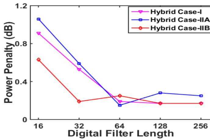
Fig. 8. Channel interference-induced power penalties for 40km upstream signal transmission for different IMDD PONs incorporating with various digital filter lengths.
