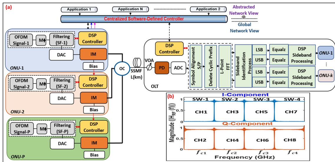
Fig. 1 (a) Schematic diagram of orthogonal digital filtering-based hybrid OFDM-DFMA PON based on IMDD (b) frequency responses of the orthogonal digital shaping filters implemented in ONUs. M \uparrow : digital up-sampling factor, SF: shaping filter, DAC/ADC: digital-to-analogue/analogue-to-digital converter. IM: intensity modulator. OC: optical coupler, PD: photo diode. S/P: serial-to-parallel conversion, LSB: lower sideband, USB: upper sideband, Equalz: equalization, ONU: optical network unit, DSP: digital signal processing, OLT: optical line terminal, SW: sub-wavelength, CH: channel.
