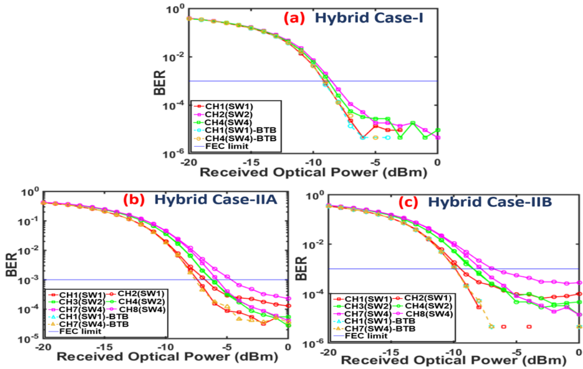
Fig. 5. BER performance versus received optical power after 40km SSMF IMDD PON transmission system subject to 0dBm optical launch power with channel bitrate of 6.25Gb/s; (a) Hybrid Case-I (b) Hybrid Case-IIA and (c) Hybrid Case-IIB. SW: sub-wavelength, CH: channel, BTB: back-to-back.
