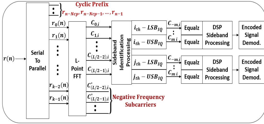
Fig. 2 Block diagram of OLT DSP procedure of the proposed PON.
