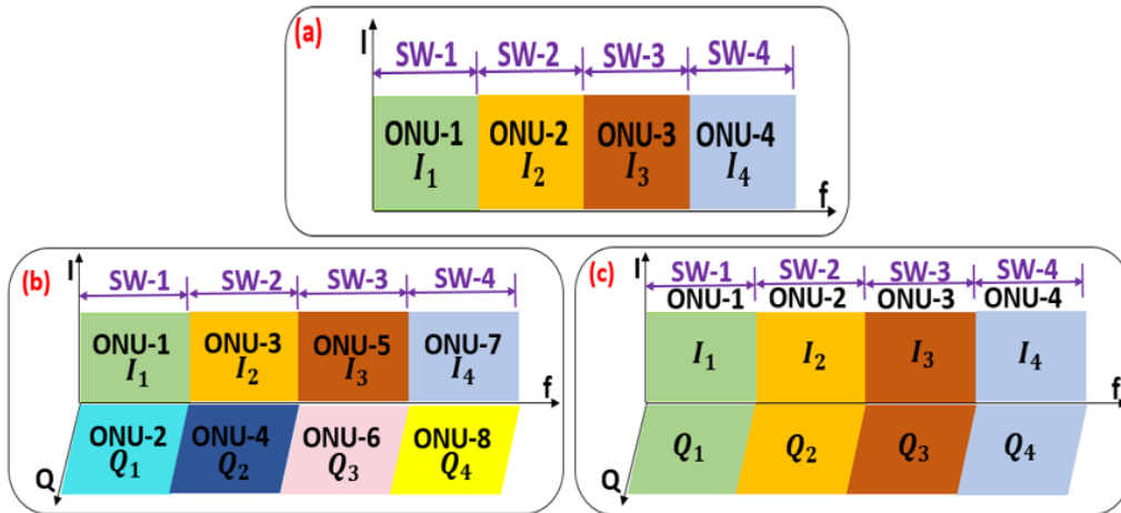
Fig. 3 Spectral locations of the digitally filtered signals in different sub-wavelength spectral region. (a) Hybrid Case-I (b) Hybrid Case-IIA and (c) Hybrid Case-IIB. SW: sub-wavelength, ONU: optical network unit, I: in-phase, Q: quadrature-phase.
