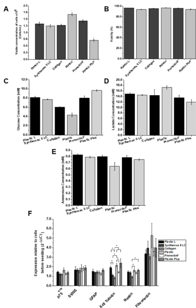
Figure 3– PA5 hOMCs were grown on Plastic L, Synthamax II LC, Collagen, Plastic, PronectinF and Plastic Plus microcarriers for 7 days with 50% media change every 2 days and using an initial seeding density of 6000 cells/cm 2 . Viable cell concentration (A) and cell viability (B) were measured. Metabolite analysis for glucose (C), lactate (D), and ammonium (E) were performed. (F) Expression of p75 NTR , S100 \beta , GFAP, \beta -III tubulin, nestin and fibronectin by PA5 hOMCs grown on Plastic L, Synthamax II LC, Collagen, Plastic, PronectinF and Plastic Plus, assessed through RT-qPCR on day 7. PA5 hOMCs before seeding were used as a reference. Data represented as mean \pm SEM, n = 3. Three independent repeats were performed for each condition. Significant differences were noted with (*) for p<0.05.
