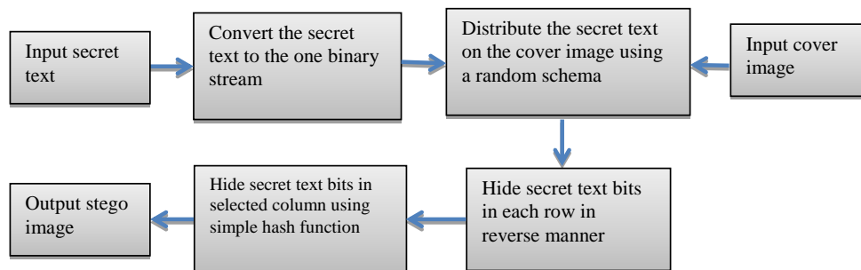
Figure 2. Proposed method processed stages
