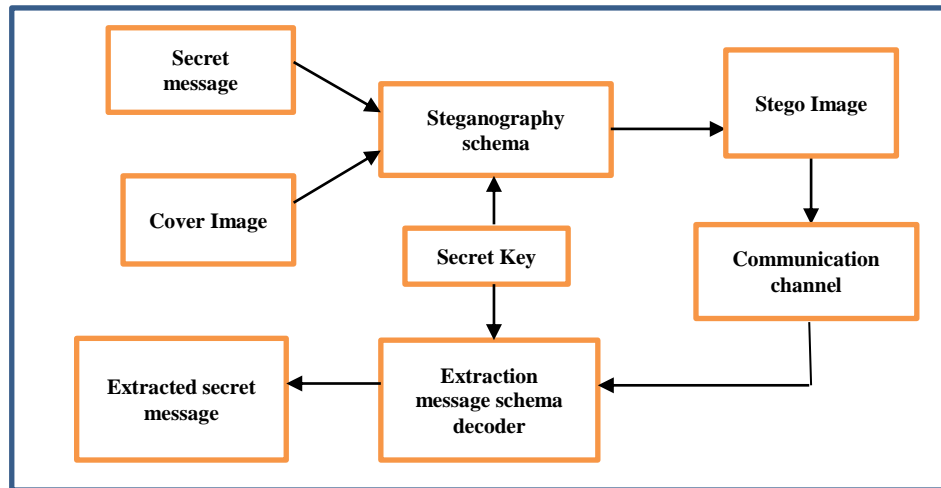
Figure 1. Basic concepts and behavior of steganography
