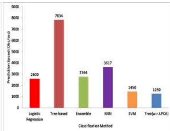
Figure 5. Comparative analysis of prediction speed
