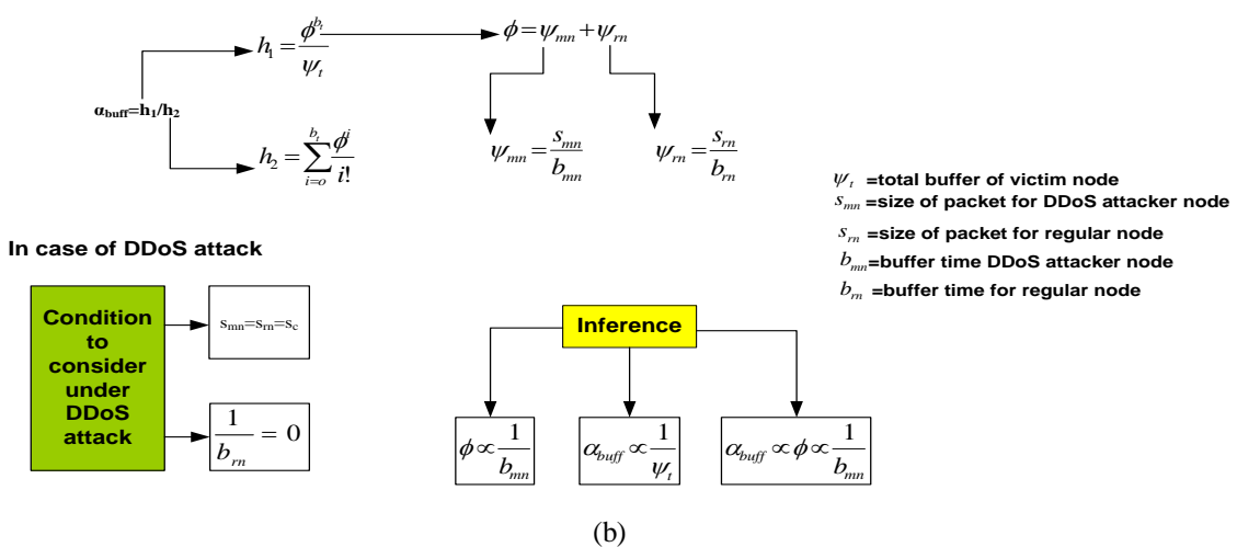
Figure 1. Extracting inference for DDoS attack in proposed system, (a) Mathematical computational flow for case-1, (b) Mathematical computational flow for case-2
