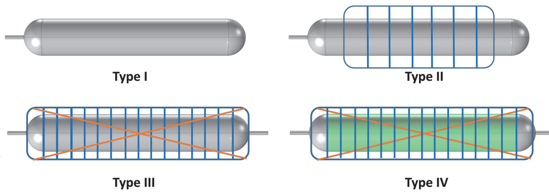
Figure 4. Hydrogen compressed gas storage, vessel types [37].
