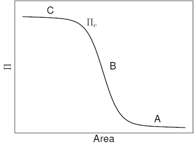
Fig. 1 Schematic of surface pressure \Pi vs area for a liquid interface laden with micron-sized particles. See the main text for an explanation of the critical surface pressure \Pi_c and the regions A, B and C (adapted from Ref. 31 ).
