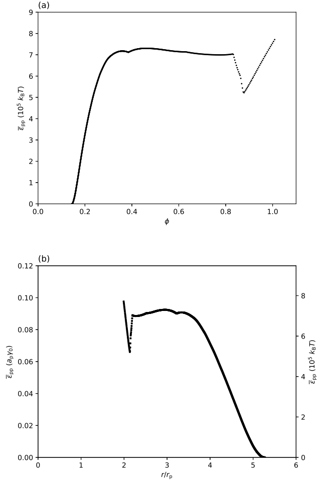
Fig. 5 (a) Interparticle potential \bar{\epsilon}_{pp} vs surface fraction \phi . (b) \bar{\epsilon}_{pp} in units of a_p \gamma_0 and in units of 10^5 k_B T vs separation r in units of particle radius r_p . These graphs were extracted from the data presented in Figure 4 using equation (26).
