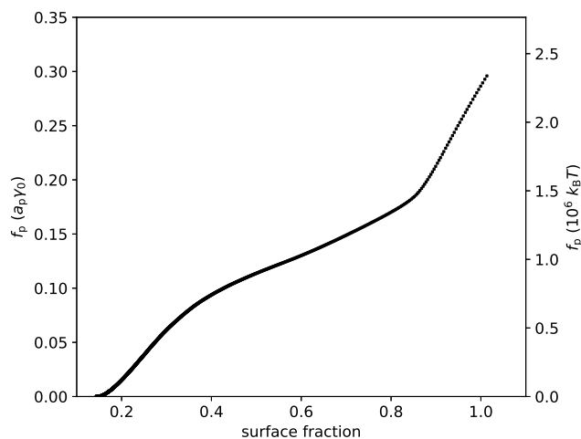
Fig. 3 Free energy per particle f_p , in units of a_p \gamma_0 and in units of 10^6 k_B T , vs surface fraction \phi . This graph was extracted from the data presented in Figure 2 using equation (23).
