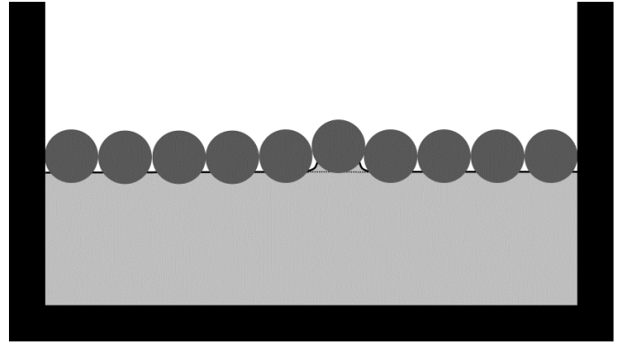
Fig. 6 Schematic of particles (dark grey) at a liquid interface (solid black line). The interfacial particles are compressed in between the vertical barriers, causing an interfacial particle to be pushed out of the plane of the initially flat liquid interface (dashed line), thereby causing a deformation of the liquid interface.
