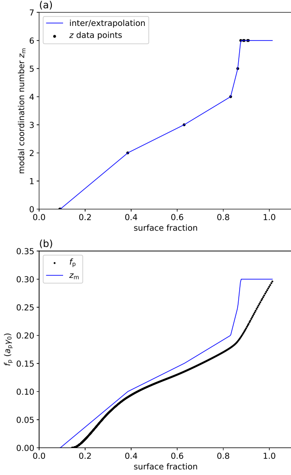
Fig. 4 (a) Modal coordination number z_m of disks on an elastic sheet vs surface fraction \phi : solid circles are data points from Ref. 45 and the solid line is a linear interpolation (apart from \phi > 0.9 where we have set z_m = 6 ). (b) Combined graph of the free energy per particle from Fig. 3 and the modal coordination number from panel (a); especially for \phi < 0.83 , the shapes of the two graphs are remarkably similar.
