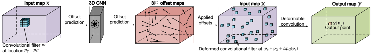
Figure 6: Graphical illustration of 3D deformable convolutional operation.
