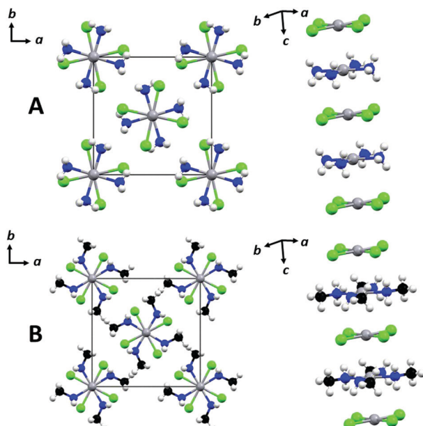
Fig. 1 Crystal packing structures of \text{MgNH}_3 (A) and \text{MgNH}_2\text{Me} (B), indicating the relationship between neighbouring salt units viewed along the [001] (left) and approximately perpendicular to the [001] (right). Atoms are coloured: Pt, dark grey; Cl, green; N, blue; C, black; H, light grey. Unit cell edges are coloured black.
